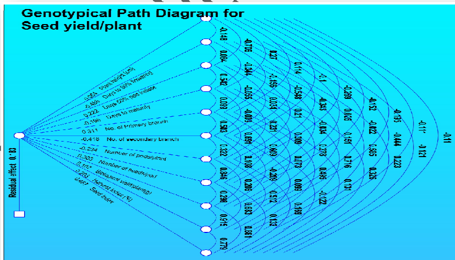
Figure 3. Genotypic Path diagram
