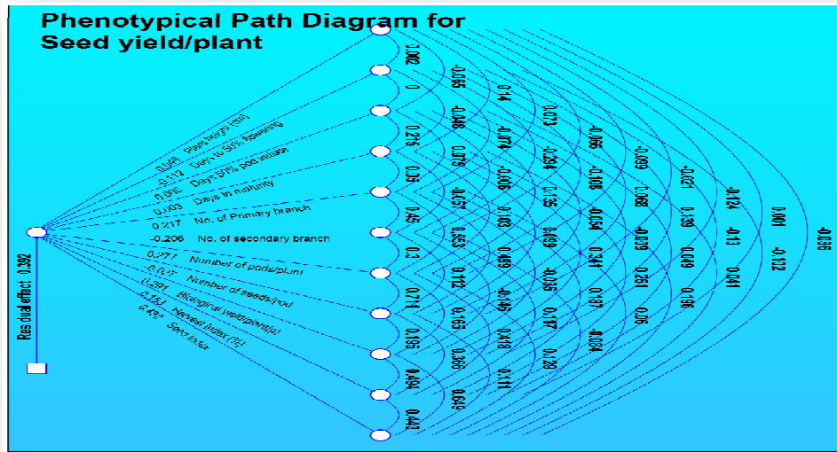
Figure 2. Phenotypic Path diagram
