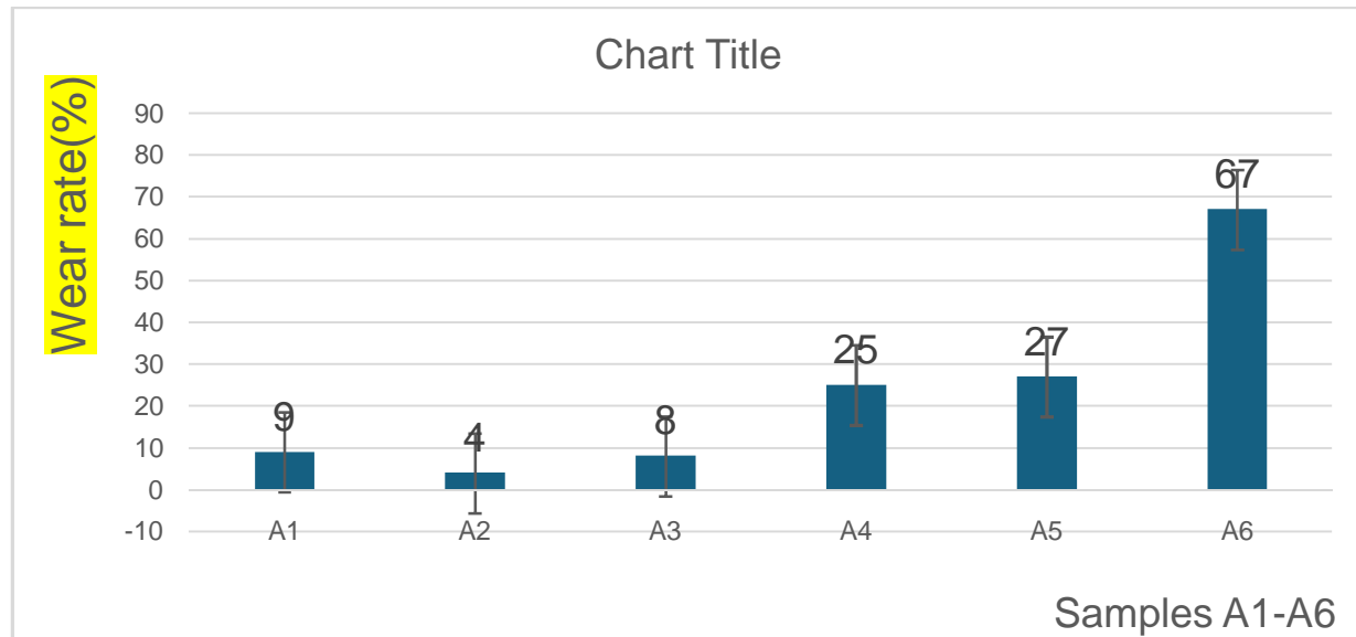
Figure 11: Variation of Wear Rate of Samples A1-A6
