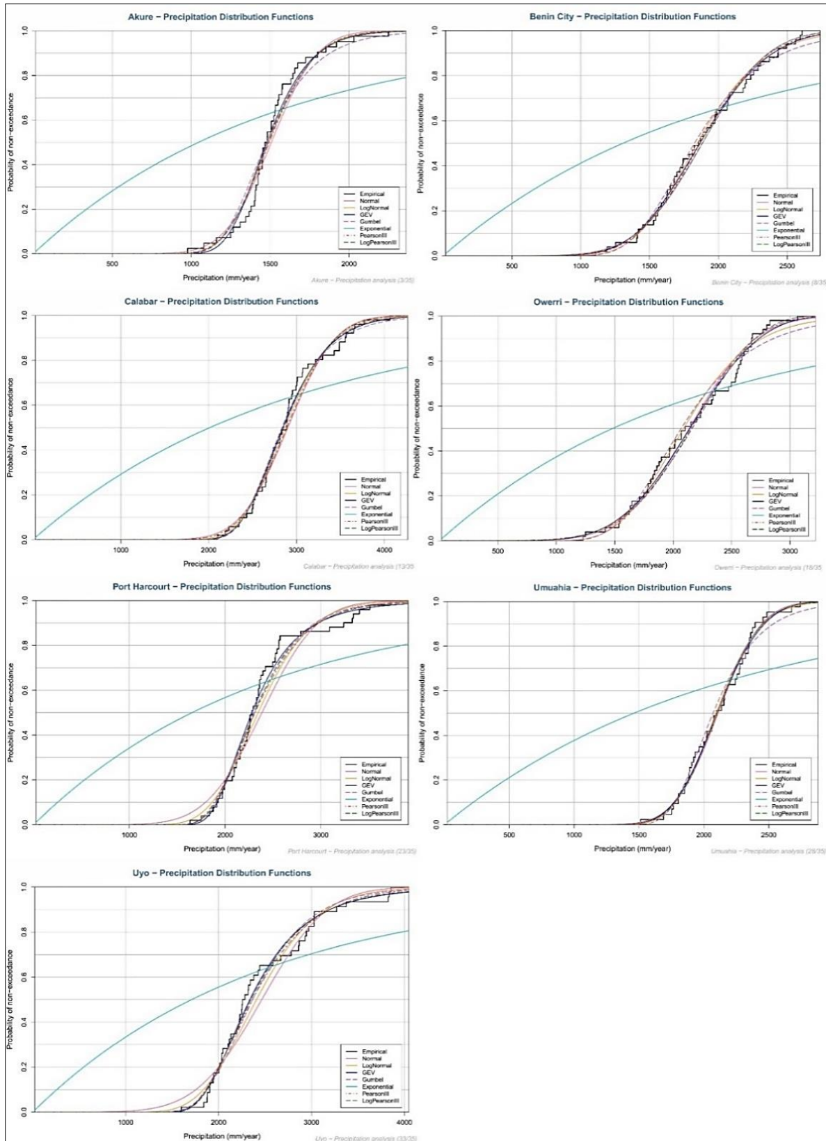
Fig. 3. Precipitation Distribution Functions for selected study stations in the Niger Delta
