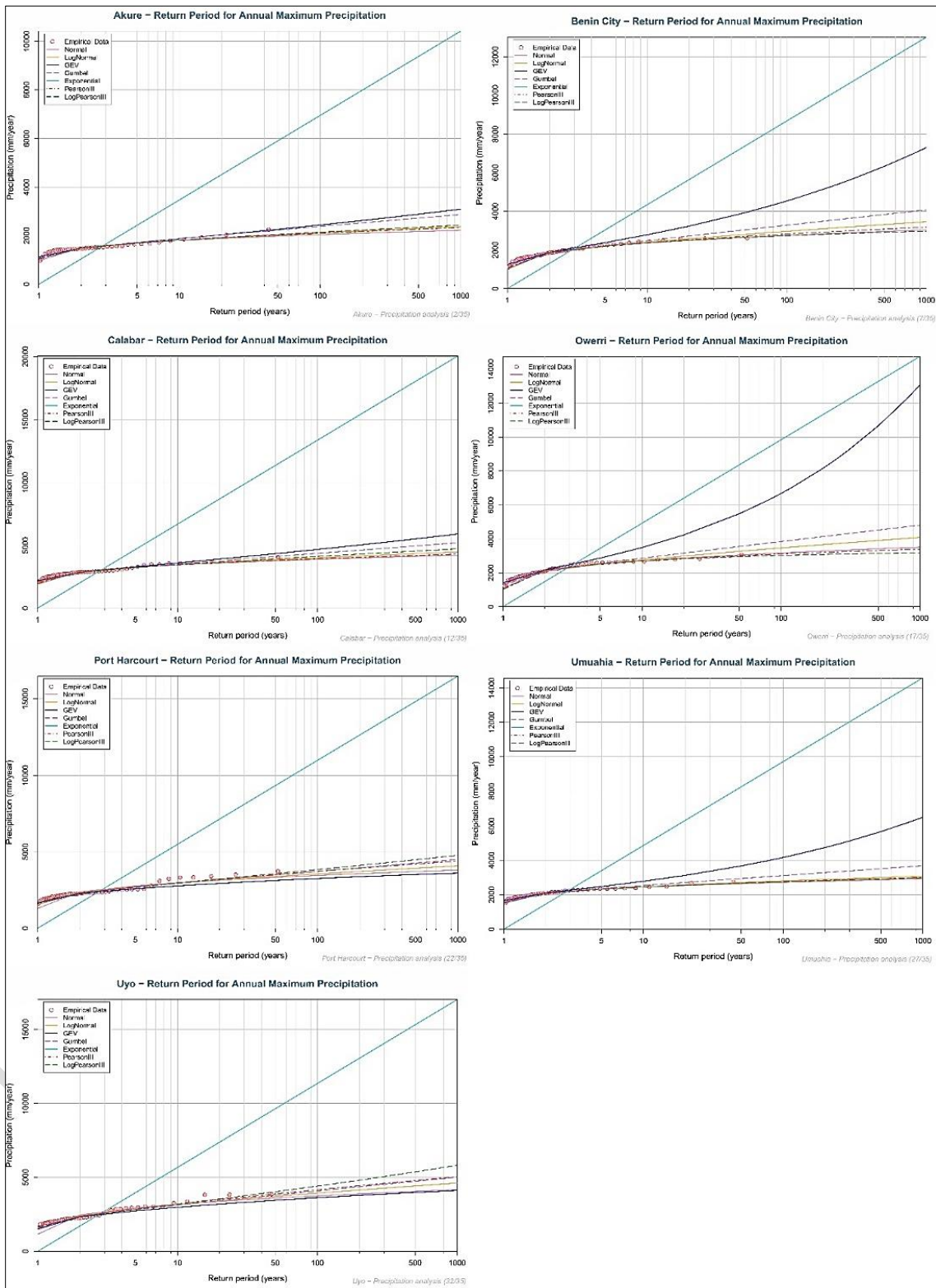
Fig. 4. Return Period Analysis for Annual Maximum Delta Precipitation for selected stations in the Niger Delta
