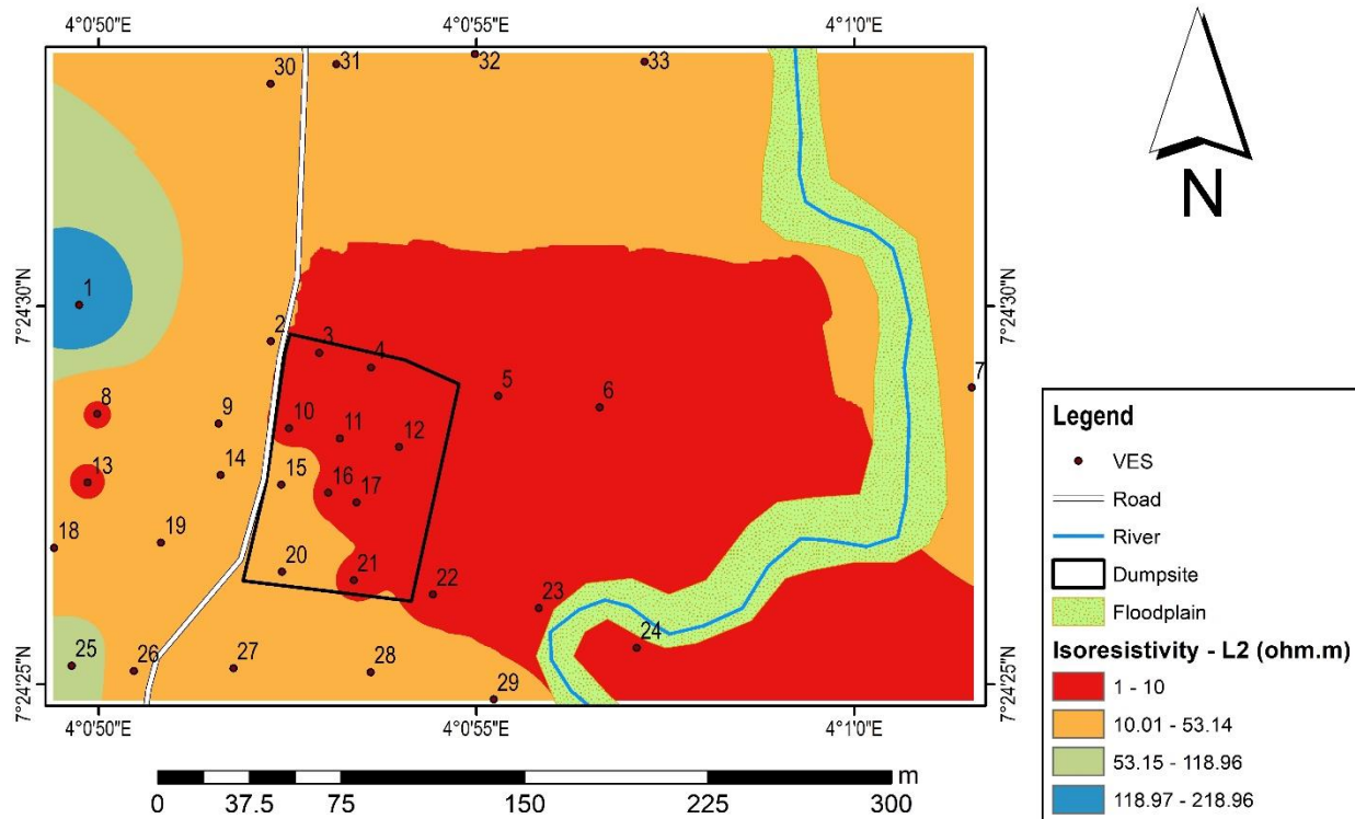
Fig. 9: Map showing the extent of contamination in the regolith beneath study area
