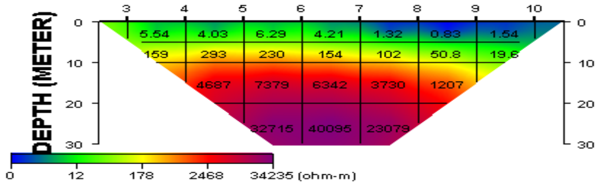
Fig. 6(a-d): 2D inverted resistivity section beneath Traverses 1-4
