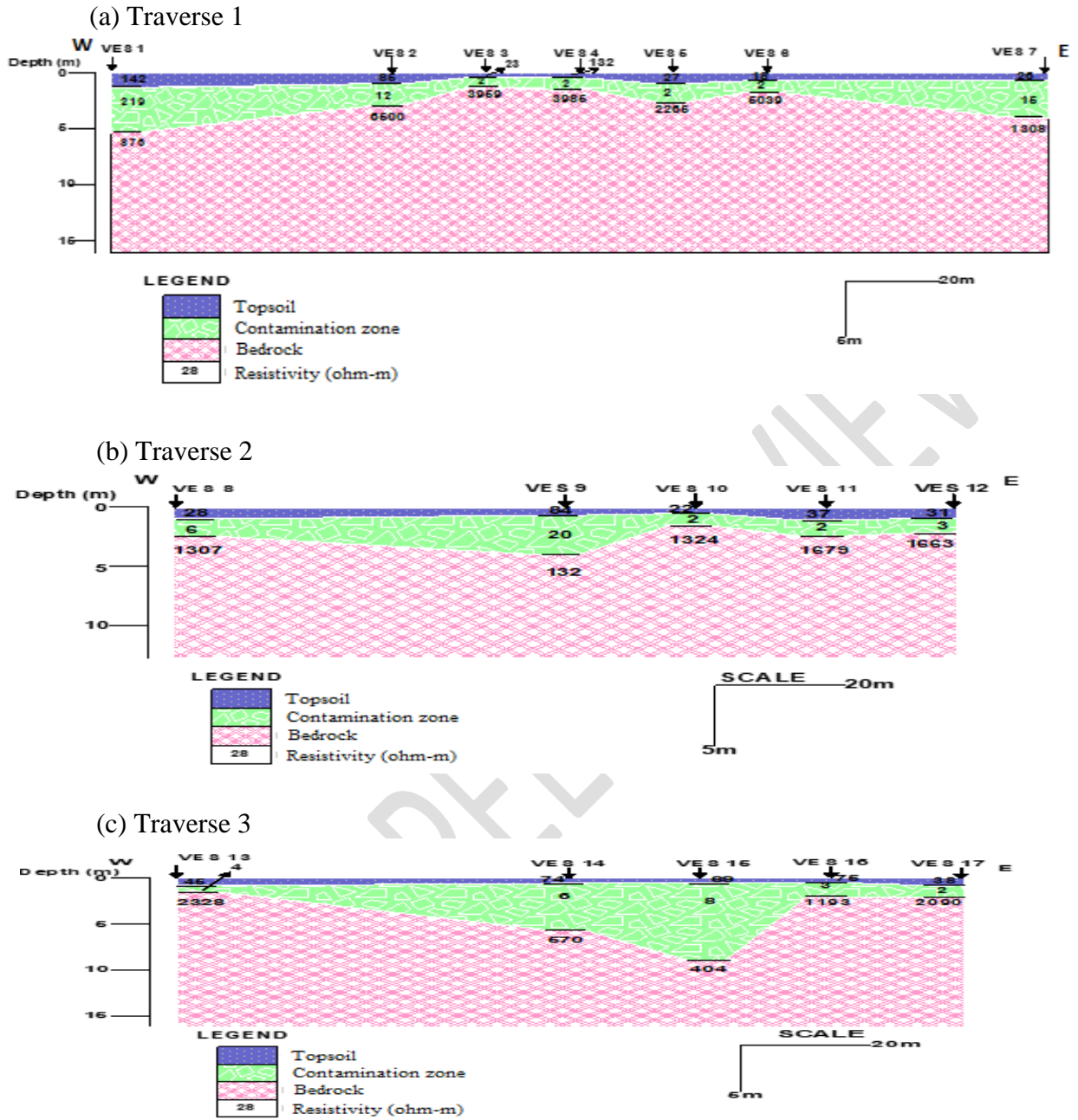
Fig. 4(a-c): Geoelectric section beneath Traverses 1- 3 in the study area
