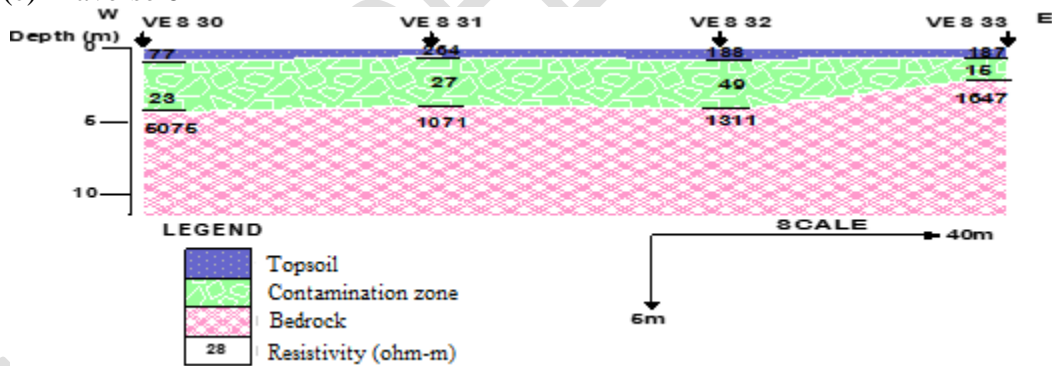
Fig. 5(a-d): Geoelectric sections beneath Traverses 4-6
