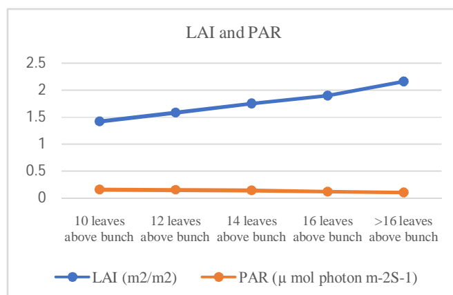
Figure 1: Effect of leaves on LAI and PAR of vine in Nanasahab Purple variety
