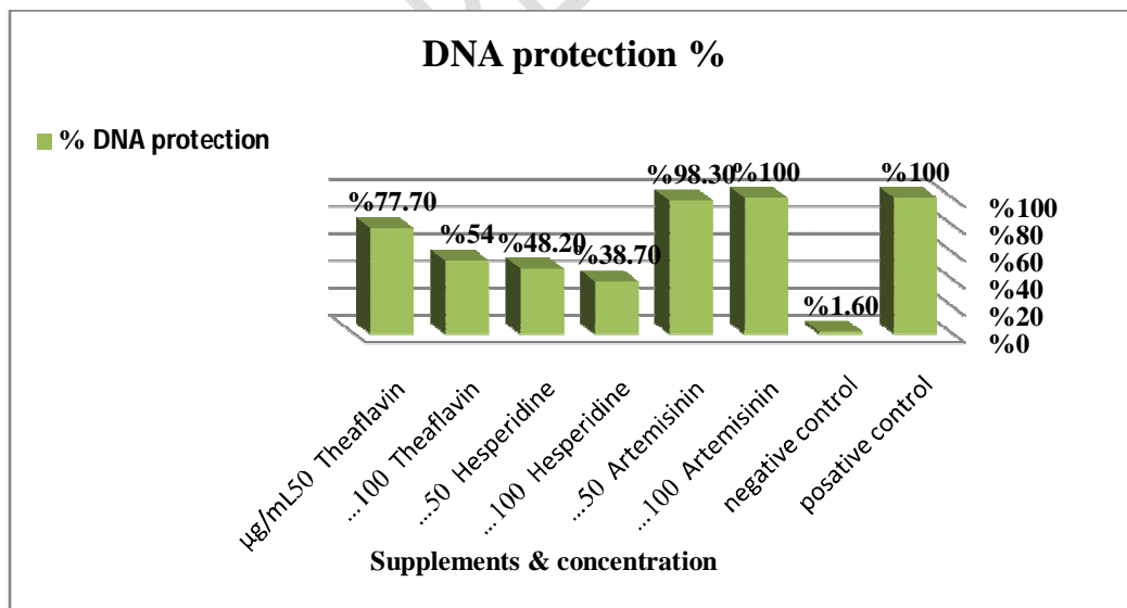
Figure 3: The human genomic DNA damage protection percent for the chosen supplements as well as the positive and negative controls.
