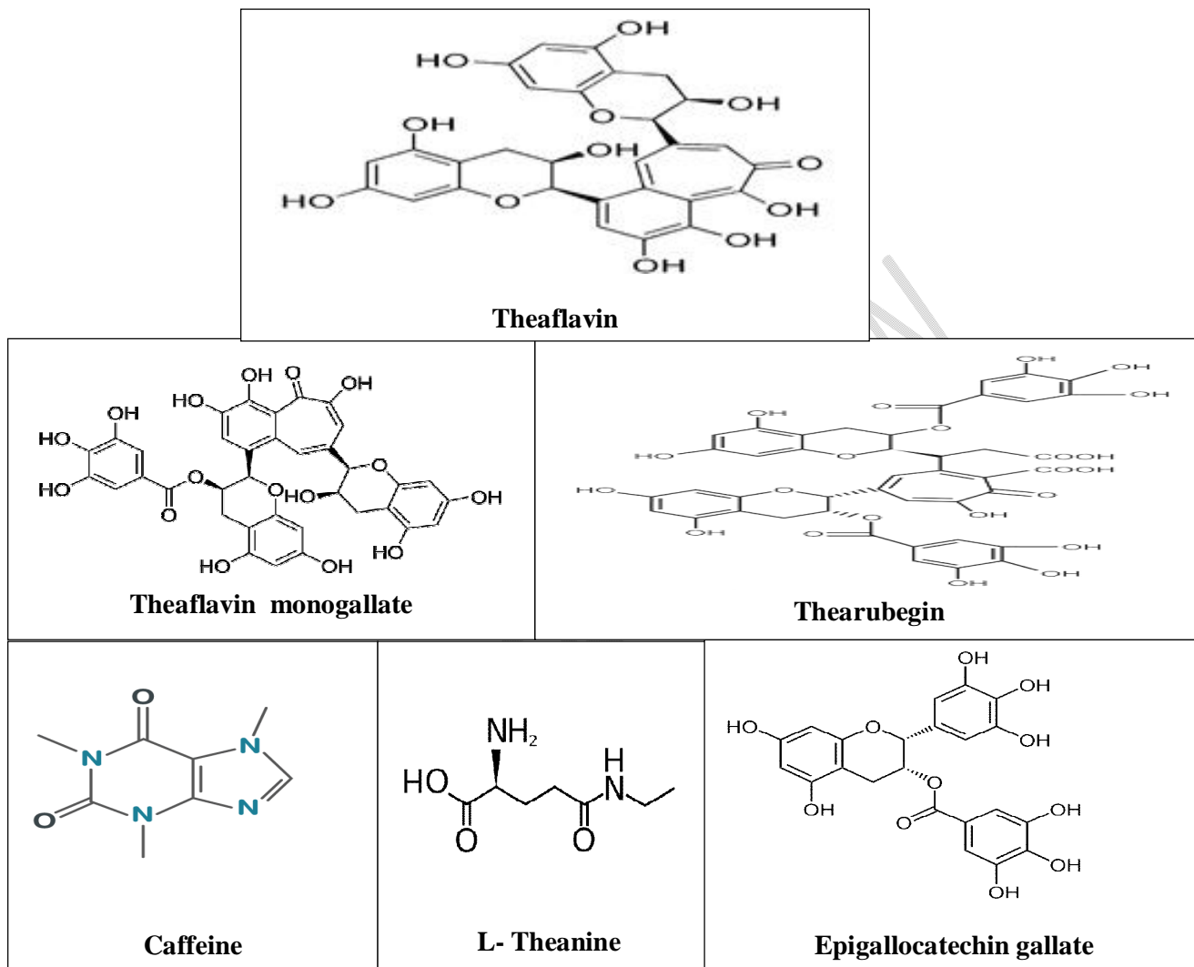
Figure 1: The name and chemical structures of the chosen compounds in the supplements.
