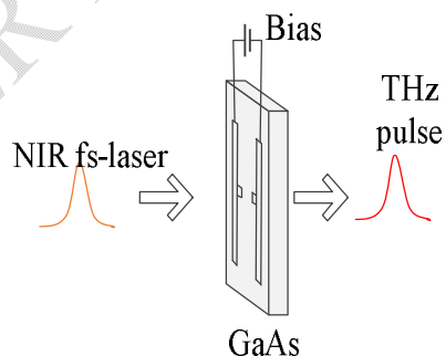
Fig. 1 Schematic diagram of terahertz radiation generated by photoconductive antenna. Optical rectification effect. Photorectification radiation is a widely used technology in the field of terahertz wave generation, whose core is the nonlinear optical effect. Light produces electron-hole pairs on the photorectifying material, and the nonlinear behavior of the material causes the current to flow in only one direction, and the light intensity changes the current size and direction, thus realizing signal modulation.
