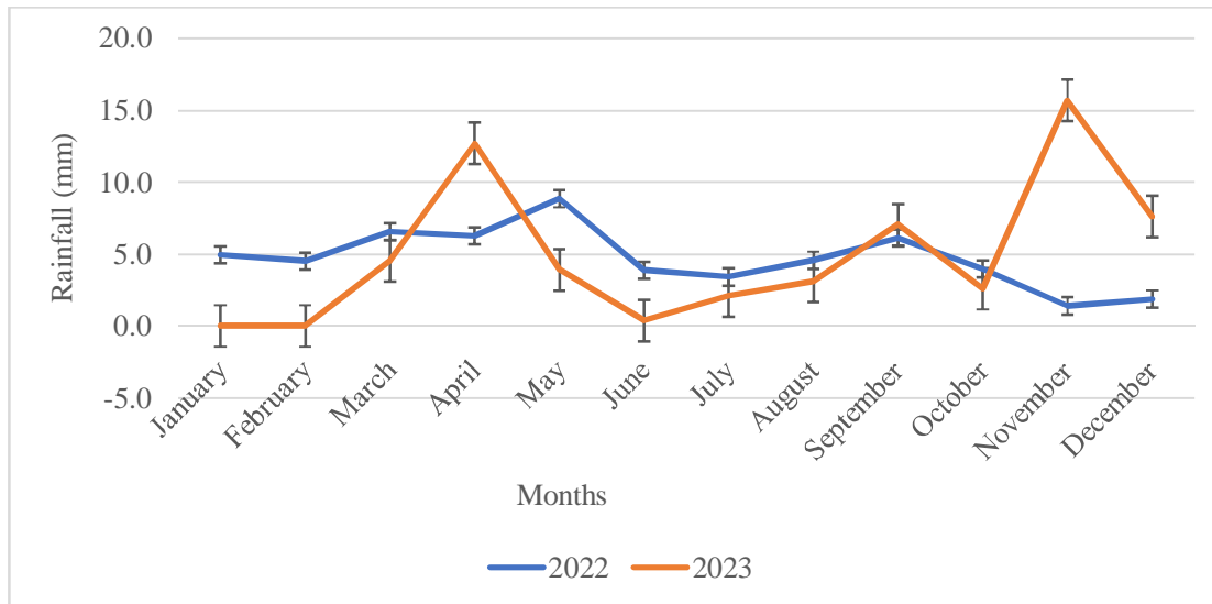
Fig. 1. The average rainfall distribution in the study area during the study period
