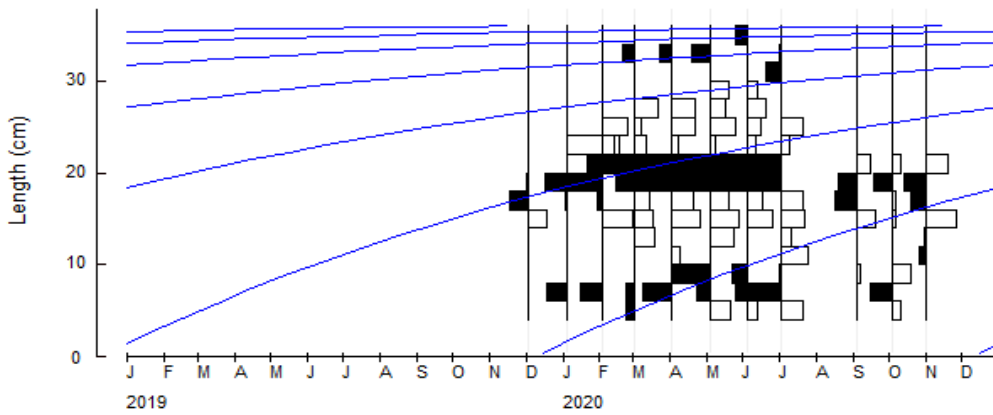
Fig. 2. Von Bertalanffy growth curve of O. niloticus by ELEFAN I based on length-frequency distribution ( L_{\infty} 36.75 cm and K 0.65 \text{yr}^{-1} ).
