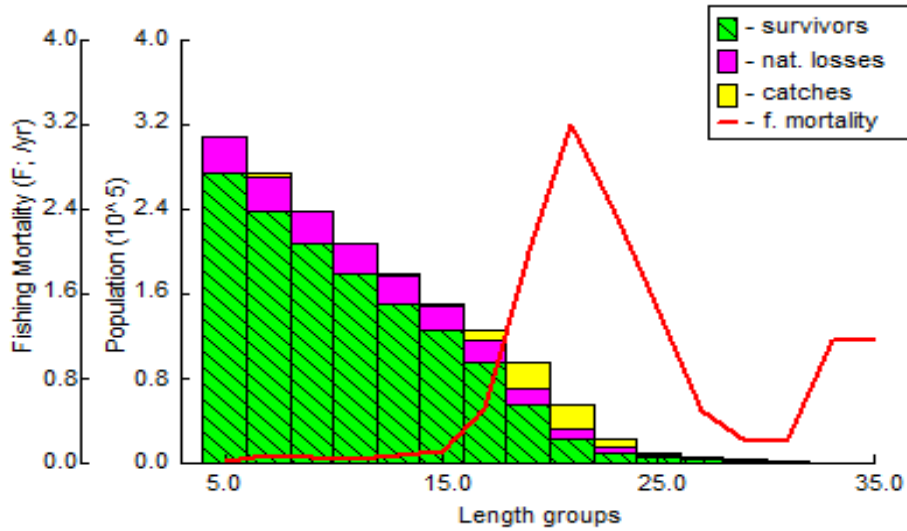
Fig. 7. Length-structured virtual population analysis of O. niloticus in Khashm El-Girba reservoir.
