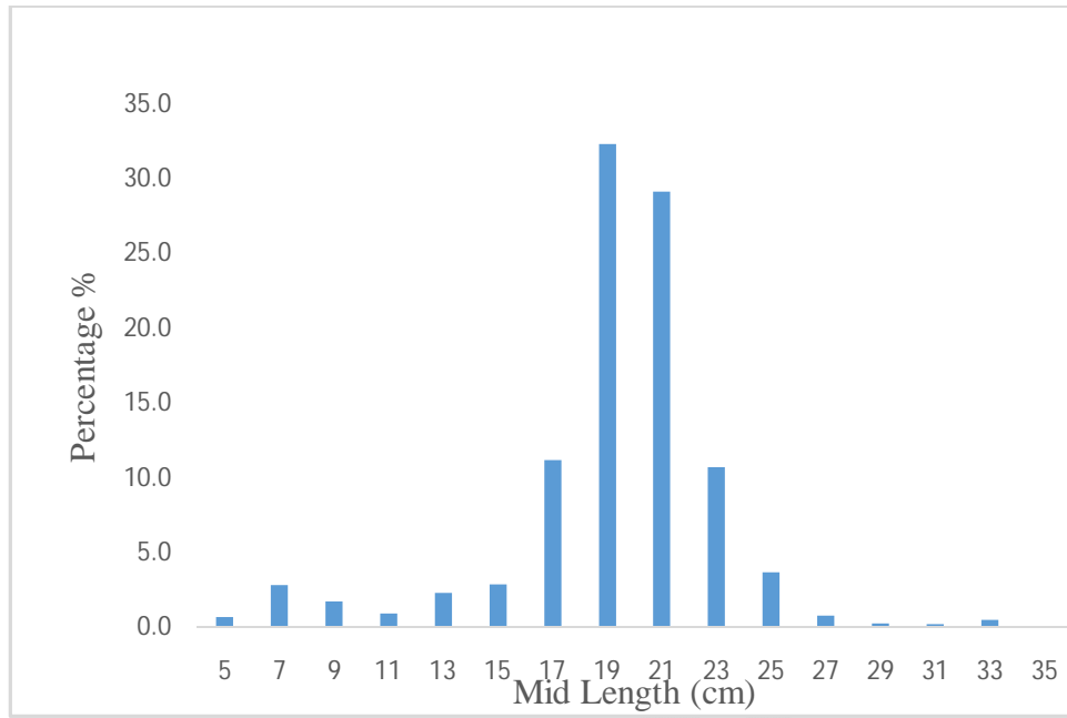
Fig. 1. Size spectrum of the Nile tilapia in Khashm El-Girba reservoir (n=1,671); Sizes are represented by the total length (cm).
