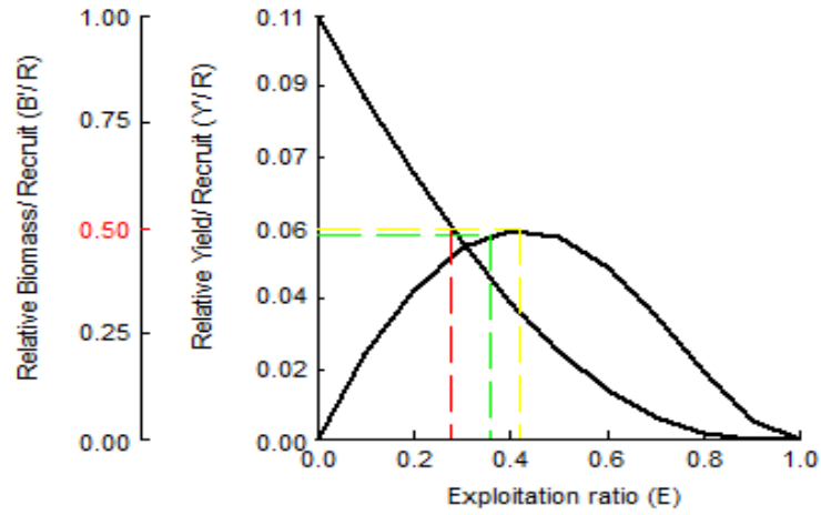
Fig. 6. Beverton and Holt relative yield per recruit (Y/R) and biomass per recruit (B/R) of the Nile tilapia in Khashm El-Girba reservoir.
