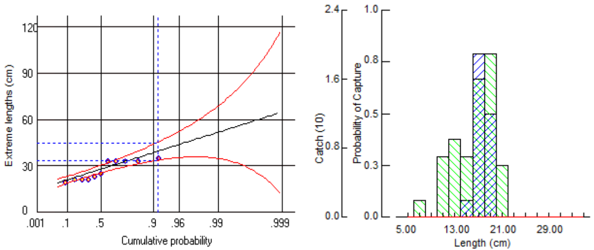
Fig. 8. Predication of a maximum of extreme length and Gillnet selection.
