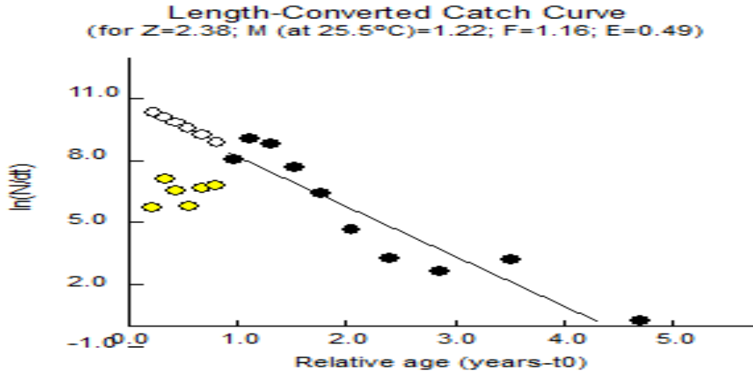
Fig. 3. Von Bertalanffy growth curve (a) ( L_{\infty}=36.75 cm; K = 0.650 yr -1 ; on length-frequency distribution and linearized length-converted catch curve of Nile tilapia in Khashm El-Girba reservoir.
