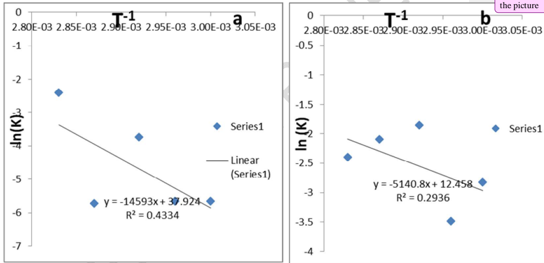
Figure 4. Plot of ln(K) against T -1 for (a) Basella alba and (b) Talinum triangulare
