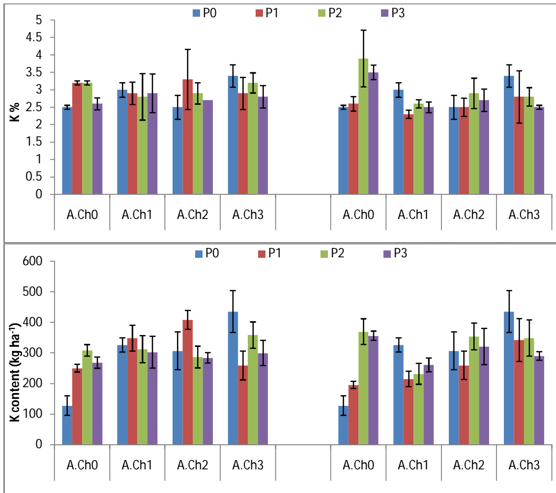
Figure (6) Potassium concentration (%) and content ( \text{kg ha}^{-1} ) in maize grains (%) as affected by phosphorus fertilizer sources, rates, and activated charcoal rates. Ph.A=phosphoric acid, S.Ph=superphosphate, A.Ch= activated charcoal
