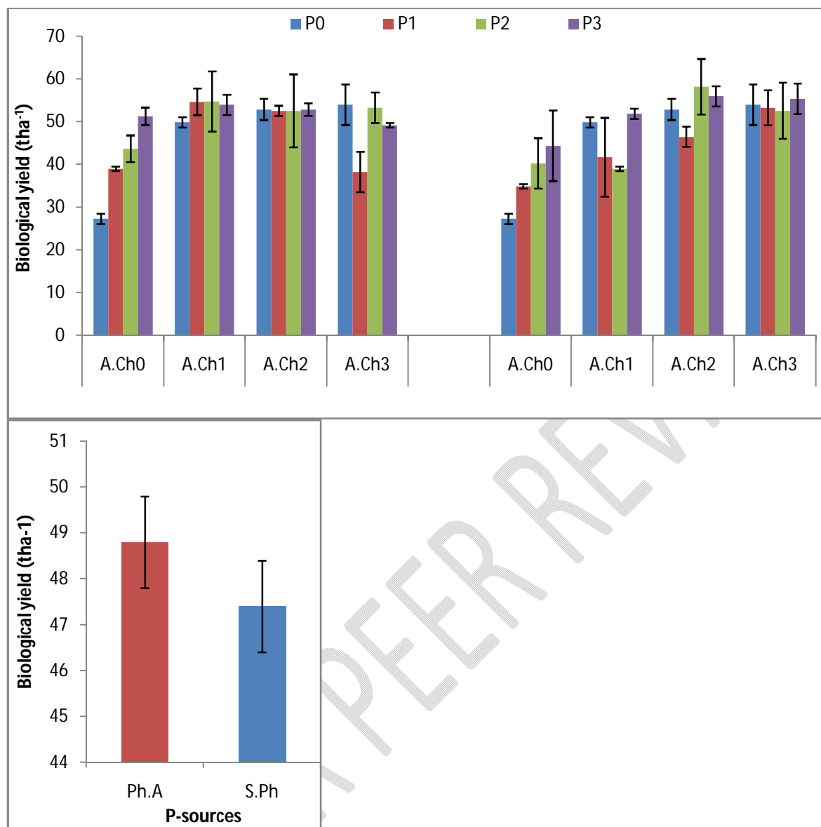
Figure (3) Biological yield( t\ ha^{-1} ) as affected by phosphorus fertilizer sources, rates, and activated charcoal rates. Ph.A=phosphoric acid, S.Ph= superphosphate, A.Ch= activated charcoal
