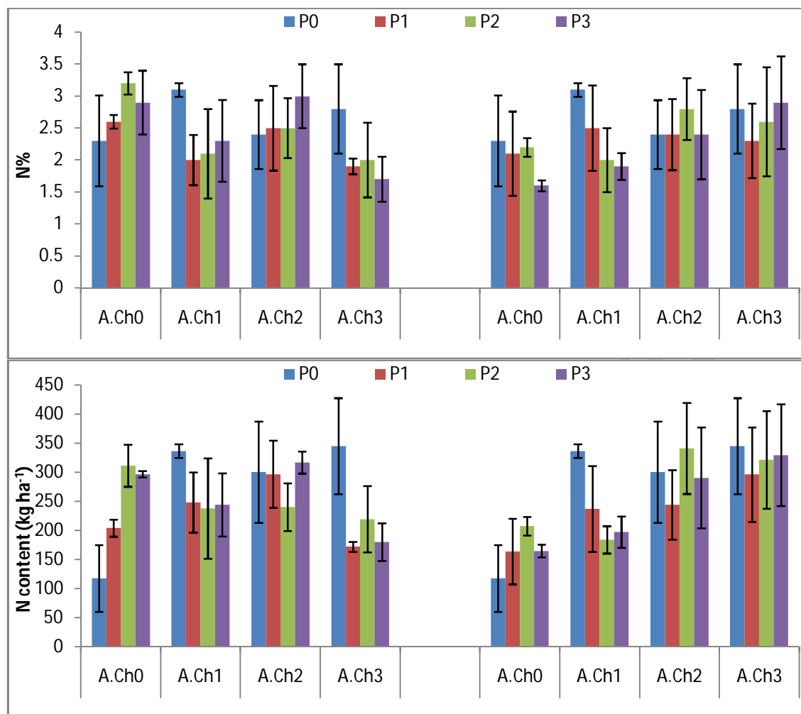
Figure (4) Nitrogen concentration (%) and content ( \text{kg ha}^{-1} ) in maize grains (%) as affected by phosphorus fertilizer sources, rates, and activated charcoal rates. Ph.A=phosphoric acid, S.Ph= superphosphate, A.Ch= activated charcoal
