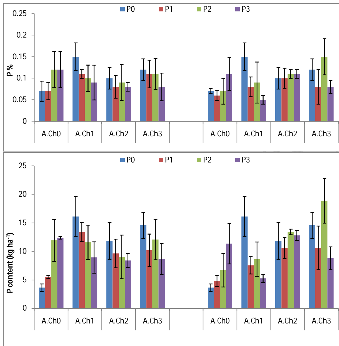
Figure (5) Phosphorus concentration (%) and content ( \text{kg ha}^{-1} ) in maize grains (%) as affected by phosphorus fertilizer sources, rates and activated charcoal rates. Ph.A=phosphoric acid, S.Ph=superphosphate, A.Ch= activated charcoal
