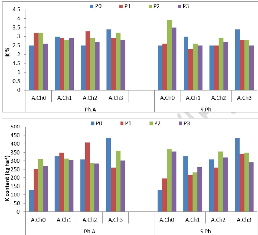
Figure 7: Potassium concentration (%) and content ( \text{kg ha}^{-1} ) in maize grains (%) as affected by phosphorus fertilizer sources, rates, and activated charcoal rates. Ph.A=phosphoric acid, S.Ph=superphosphate, A.Ch= activated charcoal
