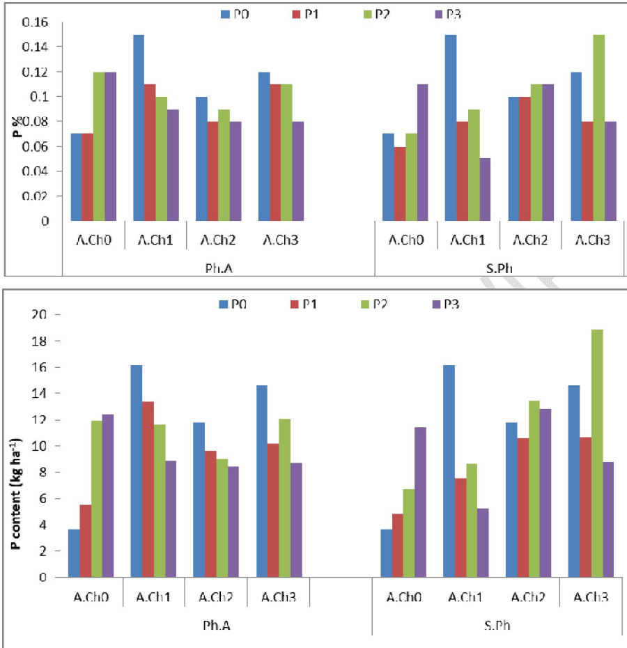
Figure 6. Phosphorus concentration (%) and content ( \text{kg ha}^{-1} ) in maize grains (%) as affected by phosphorus fertilizer sources, rates and activated charcoal rates. Ph.A=phosphoric acid, S.Ph=superphosphate, A.Ch= activated charcoal
