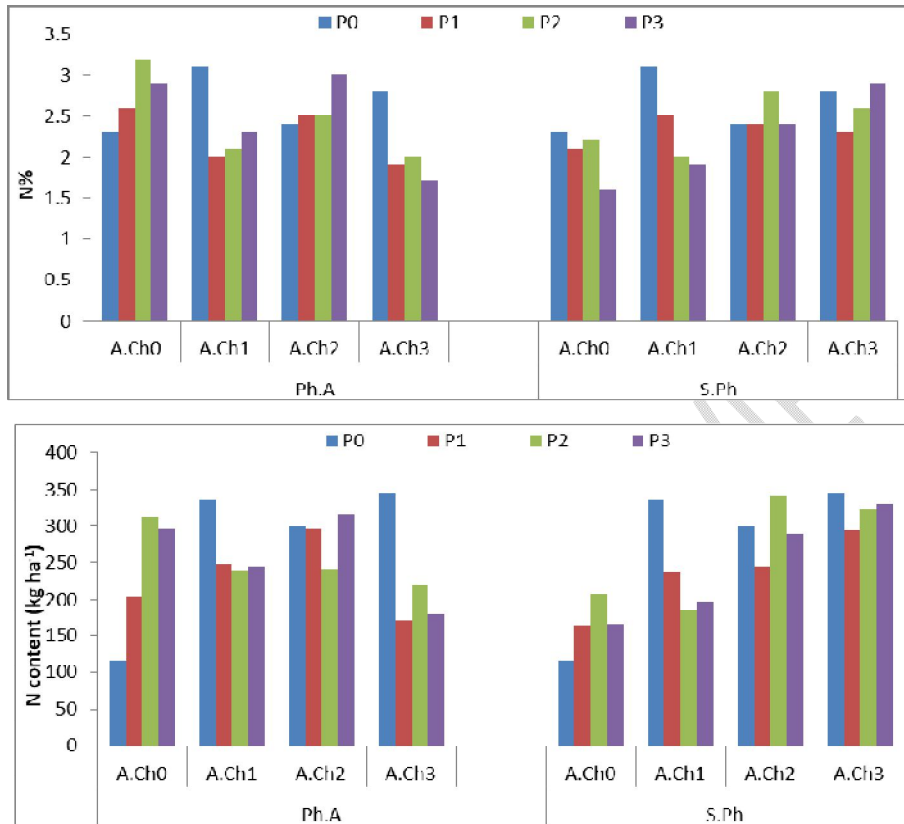
Figure 5 Nitrogen concentration (%) and content (kg ha -1 ) in maize grains (%) as affected by phosphorus fertilizer sources, rates, and activated charcoal rates. Ph.A=phosphoric acid, S.Ph=superphosphate, A.Ch= activated charcoal
