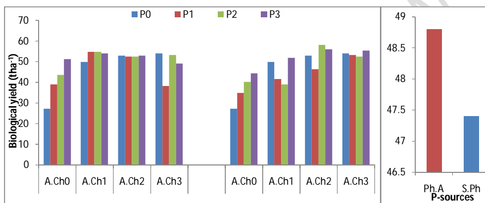
Fig. (3) Biological yield( t\ ha^{-1} ) as affected by phosphorus fertilizer sources, rates, and activated charcoal rates. Ph.A=phosphoric acid, S.Ph= superphosphate, A.Ch= activated charcoal
