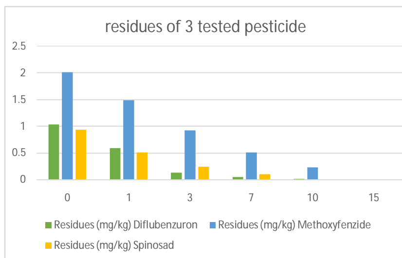
Fig (2) Residues effect of Spinosad, methoxyfenzide and diflobezuron on tomato fruits during 15 days
