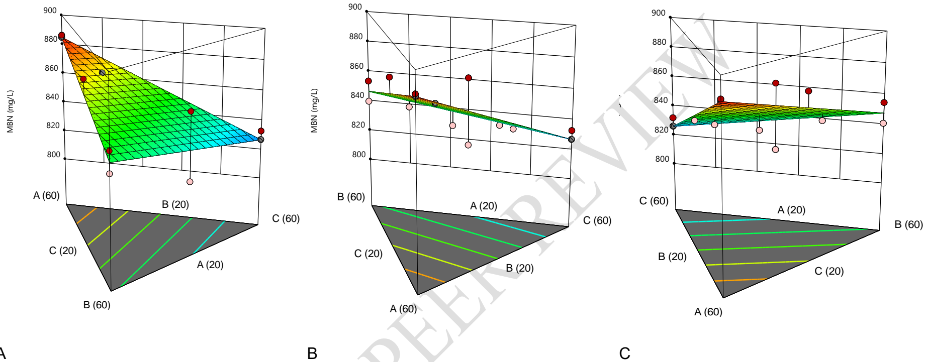
Fig. 5. 3D plot of Composition ranges of the H_3PO_4 -modified, NaOH-modified and BaCl_2 -modified Almond Shells on the MBN
