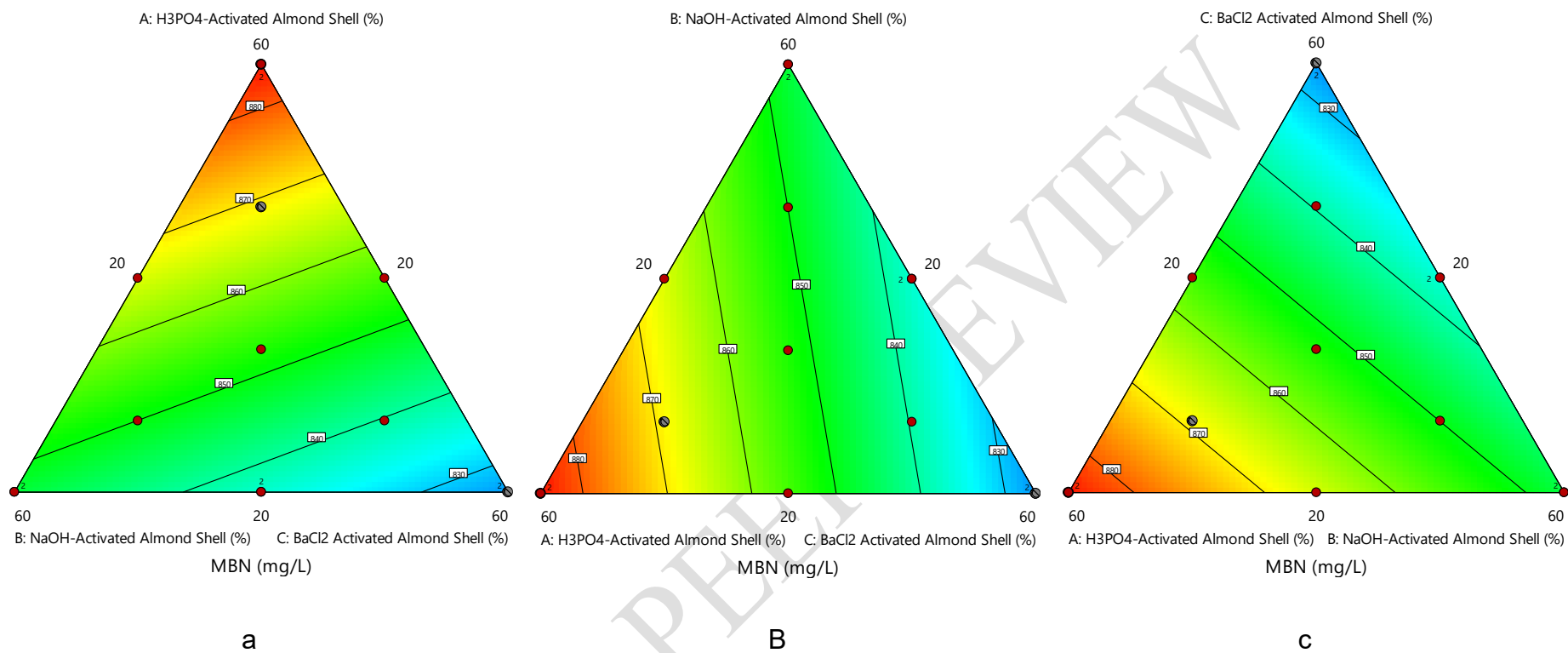
Fig. 4. Contour plot of Composition ranges of the H 3 PO 4 -modified NaOH-modified and BaCl 2 modified Almond Shells on the MBN
