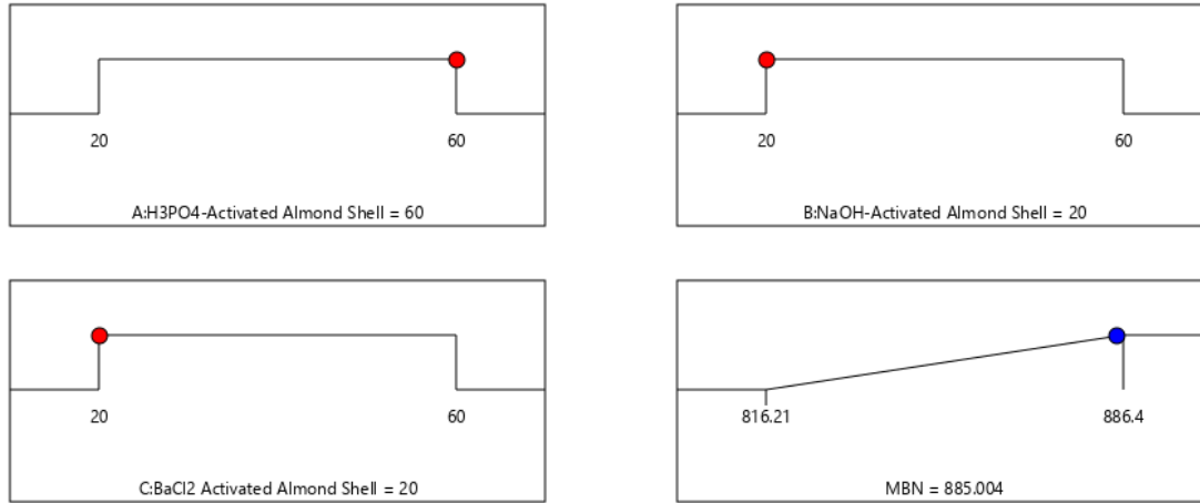
Fig. 6: Numerical Optimum value for the tricomposite composition
