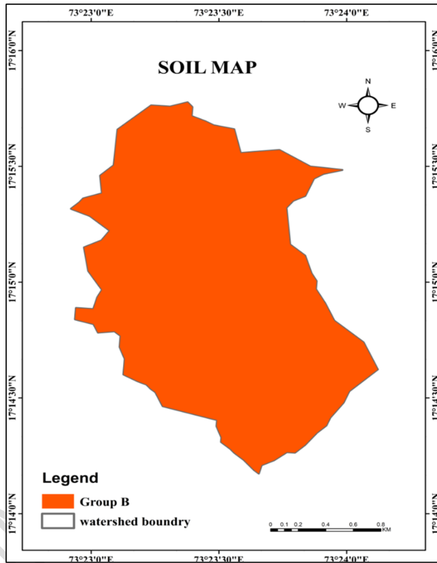
Fig. 4 Hydrological soil group map of Kajurli watershed
