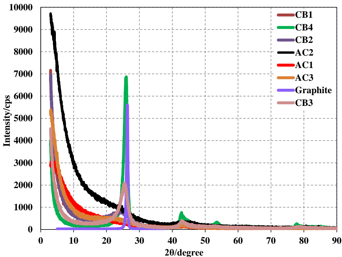
Figure 6. The integrated X-ray diffraction spectra for all the three ACs and four CBs. The diffraction datasets for the graphite are also plotted for comparison purpose.
