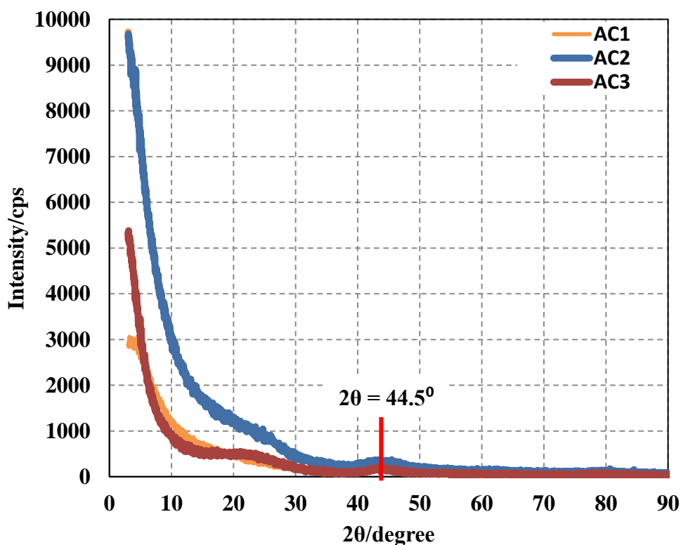
Figure 1. The X-ray diffraction spectra for activated carbon samples AC1, AC2, and AC3 carbonized at \sim 600 – 900^\circ\text{C} .
