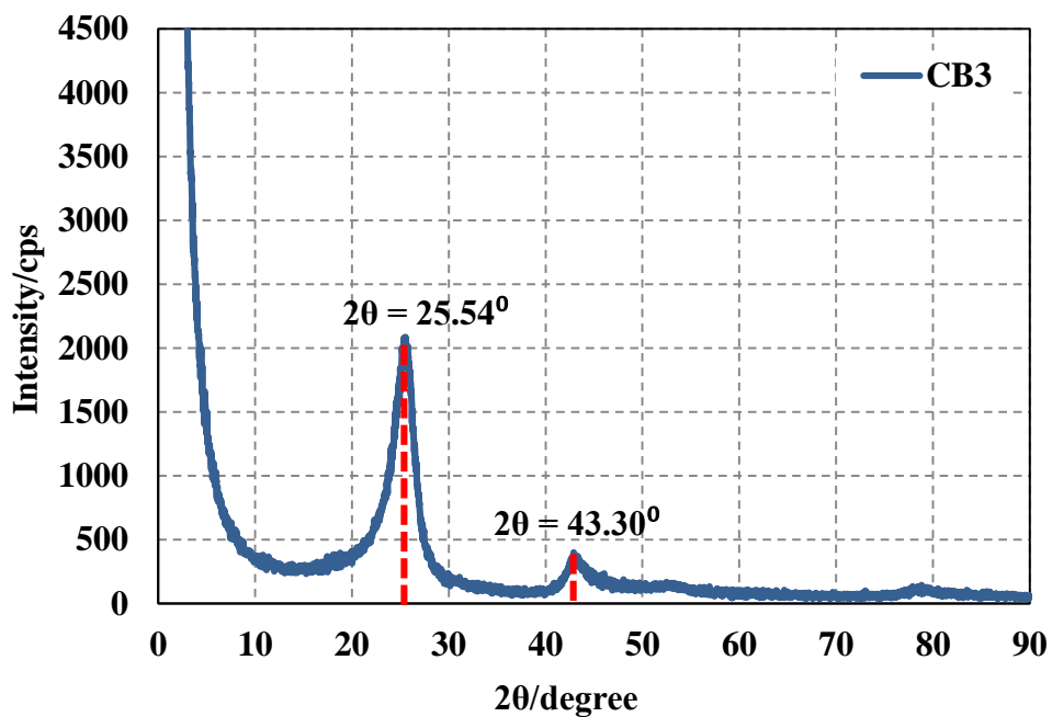
Figure 4. The X-ray diffraction spectrum for carbon clack CB3 graphitized at \sim 2000^{\circ}\text{C} .
