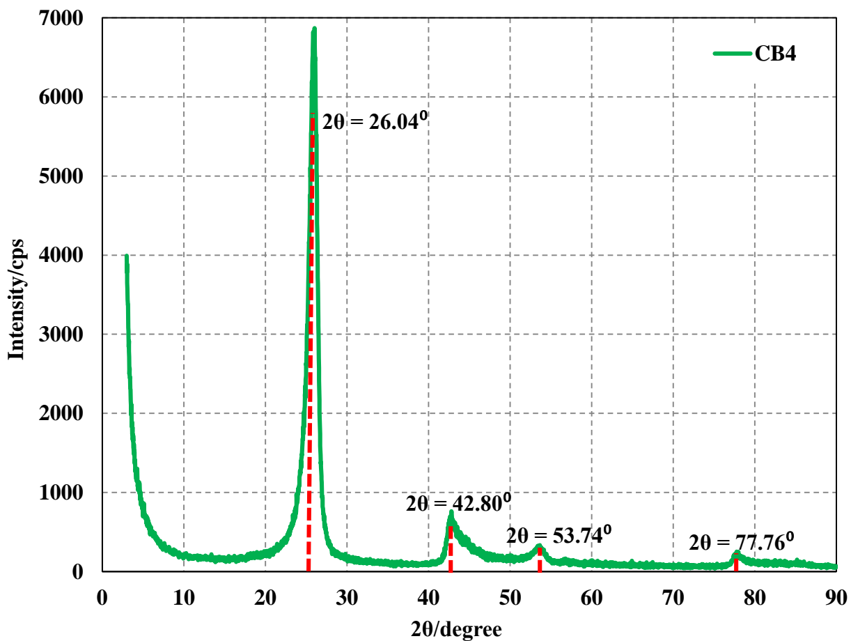
Figure 5. The X-ray diffraction spectrum for carbon clack CB4 graphitized at > 2500^{\circ}\text{C} .
