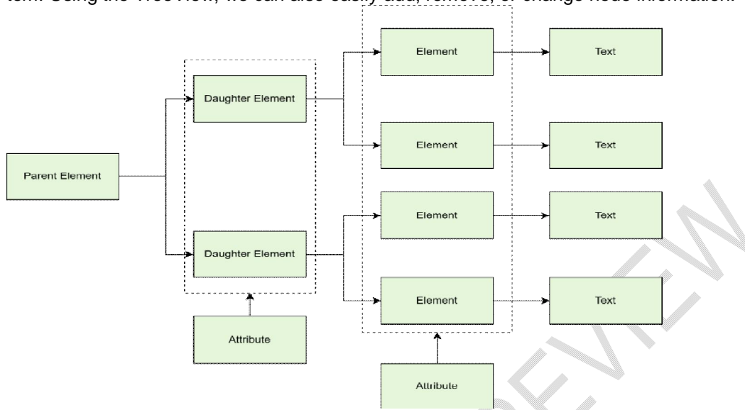
Figure 5. TreeView element structure
