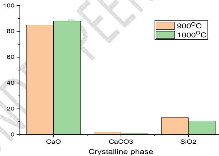
Figure 6: Effect of calcination temperature on crystalline phase of CaO-based biocatalyst.
