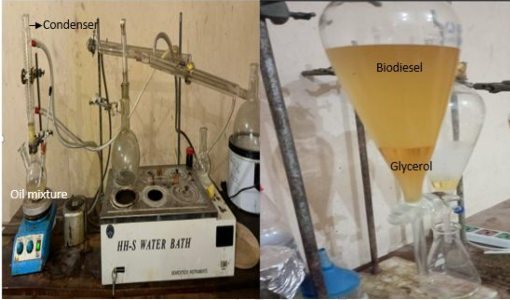
Figure 2. (a) Transesterification set-up, (b) Biodiesel mixture
