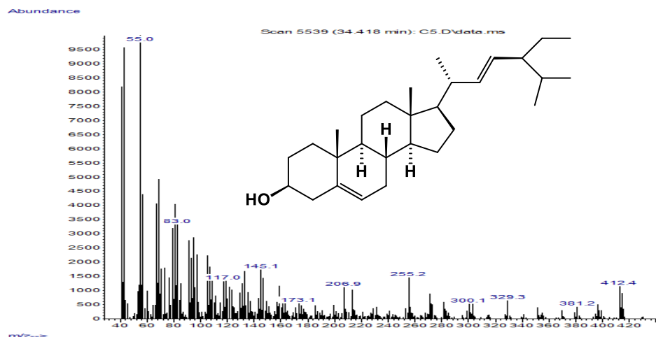
Fig. 3: GC-MS spectrum of C5
