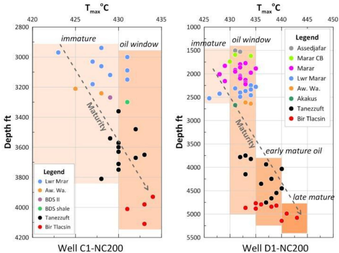
Fig. 5. The T_{max} maturity parameter of the samples collected from the C1- and D1-NC200 wells shows that the samples of Silurian Source rocks located at the oil window at least, while the Devonian Carboniferous Sources wereshowing that the samples of Silurian Source rocks located at the oil window at least, while the Devonian Carboniferous Sources was immature to the oil window maximum.
