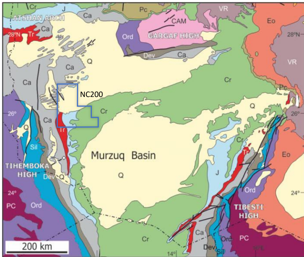
Fig. 1. Geological map of Murzuq basin showing the major stratigraphic units, the basin boundaries, and the location of the Erwin oil field (NC 200) modified from 15 . PC= Precambrian; CAM=Cambrian; Ord=Ordovician; Sil=Silurian; Dev; Devonian; Ca= Carboniferous; Tr= Triassic; J= Jurassic; Cr=Cretaceous; Pc=Paleocene; Eo=Eocene; VR= Tertiary volcanic rocks; and Q=Quaternary.
