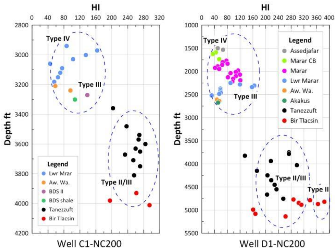
Fig. 4. The HI values of the selected samples from both C1- and D1-NC200 wells plotted verses-versus versus the depth showing the Silurian sources are mostly represented by type II/III kerogen and minor type II kerogen (in D1-NC200, particularly), whereas the . In contrast, type III and IV kerogen dominate the Devonian-Carboniferous source rocks Devonian-Carboniferous source rocks are dominated by type III and IV kerogen.
