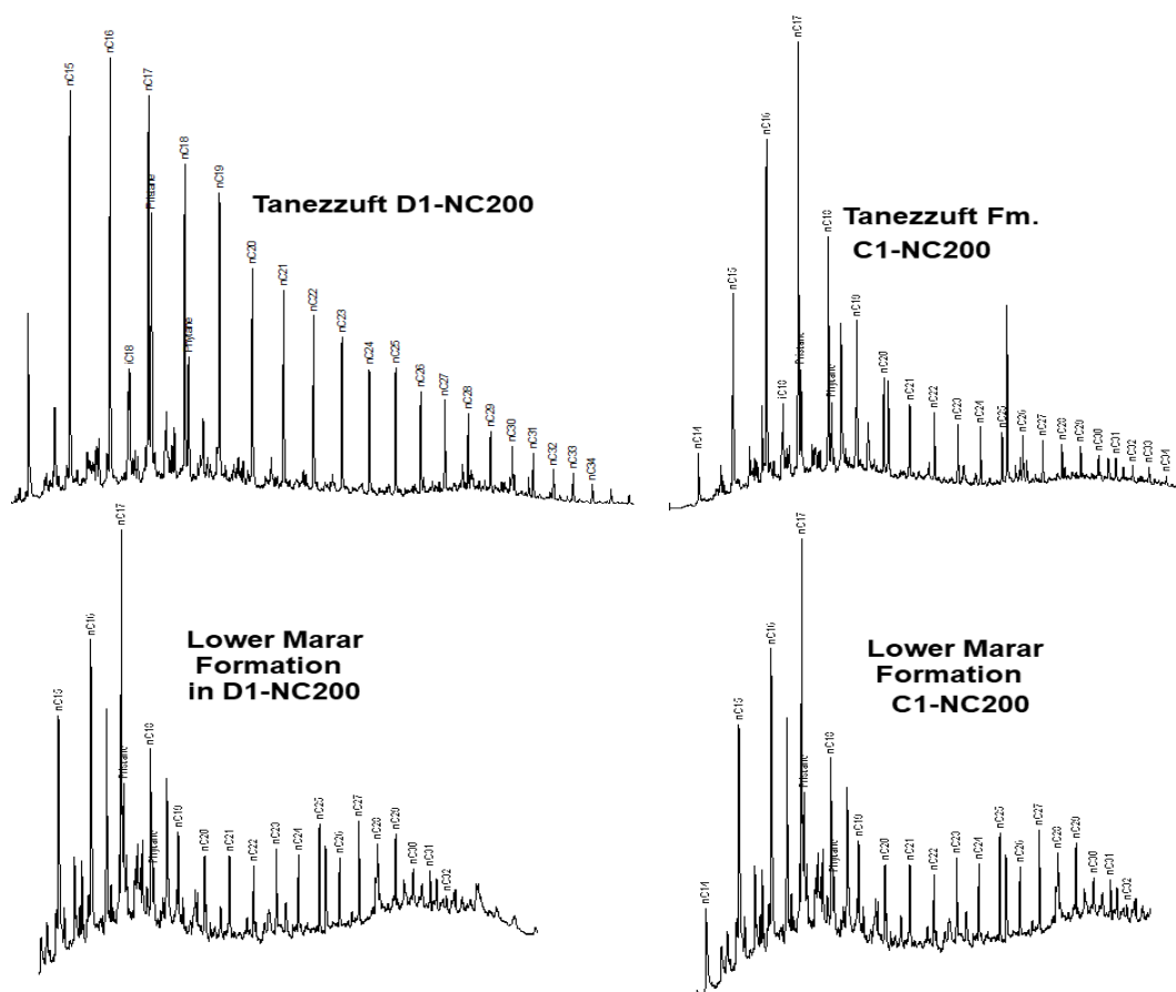
Fig. 6. shows the GC-MS profile of samples from the C1 and D1-NC200 wells of the Silurian (Tanezzuft) and Devonian (Lower Marar) formations, indicating shows the GC-MS profile of samples from the C1 and D1-NC200 wells of the Silurian (Tanezzuft) and Devonian (Lower Marar) formations. This indicates that the n -C20 and isoprenoids (Pristane & Phytane) exhibit similar patterns to other regular n -alkanes.
