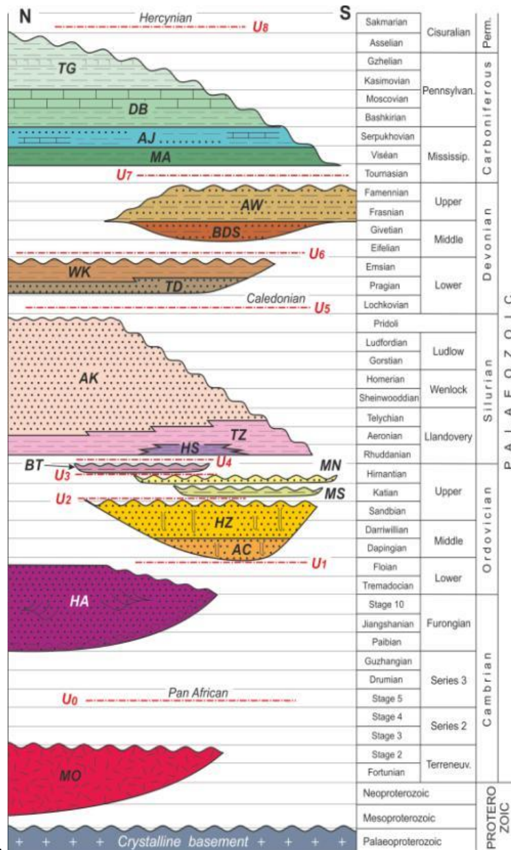
Fig. 2. Generalized chronostratigraphic section of the Murzuq Basin showing the major lithostratigraphic units and their major unconformities (adopted from 15 ). MO = Mourizide; HA = Hasawnah; AC = Achabiyat; HA = Hawaz; MS = Melaz Shuqran; MN = Mamuniyat; BT = Bir Tlacin; HS = Hot Hale; TZ = Tanezzuft; AK = Akakus; TD = Tadrart; WK = Wan Kasa; BDS = Basal Devonian Sandston; AW = Awaynat Wanin; MA = Marar; AJ = Assedjefar; DB = Dembaba; TG = Tiguentourine; and U1-U6 = major unconformities.
