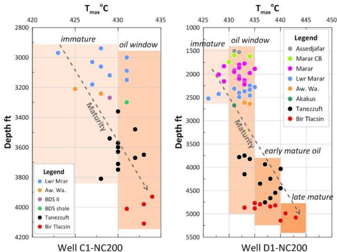
Fig. 5. The T_{max} maturity parameter of the samples collected from the C1- and D1-NC200 wells showing that the samples of Silurian Source rocks located at the oil window at least, while the Devonian Carboniferous Sources was immature to the oil window maximum.
