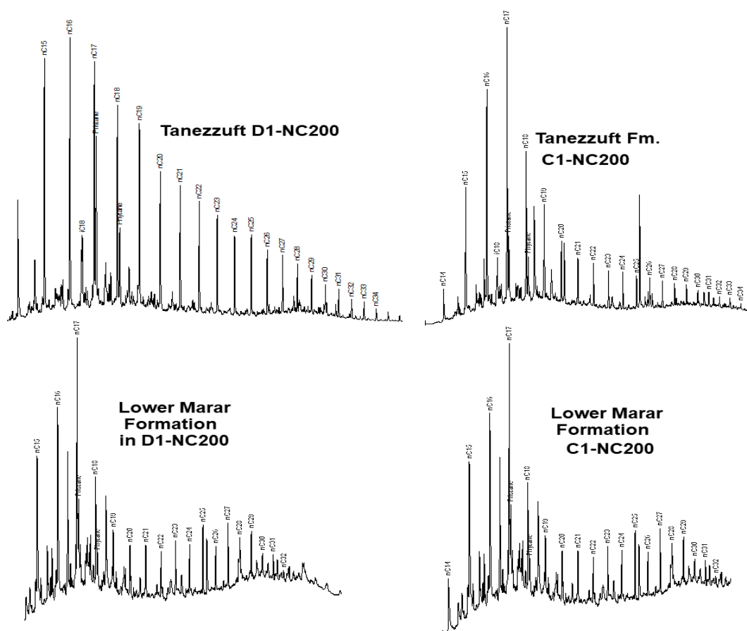
Fig. 6. shows the GC-MS profile of samples from the C1- and D1-NC200 wells of the Silurian (Tanezzuft) and Devonian (Lower Marar) formations, indicating that the n -C20 and isoprenoids (Pristane & Phytane) exhibit similar patterns to other regular n -alkanes.
