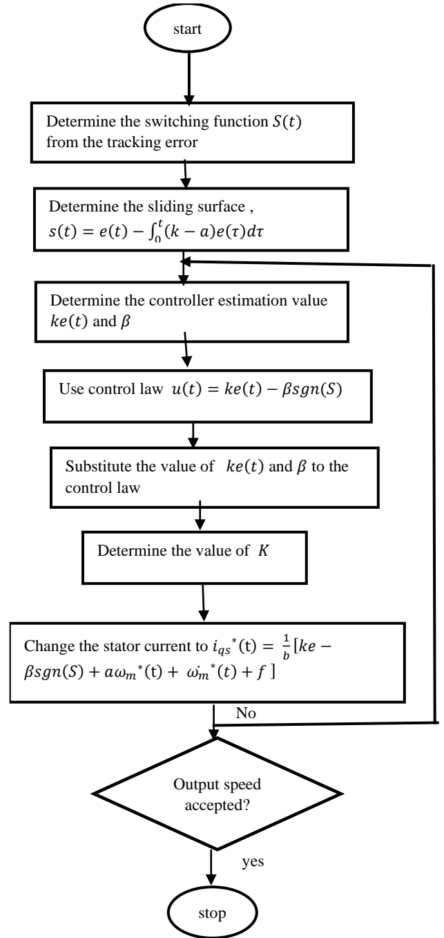
Figure 2: flow chat of slidng mode controller development
