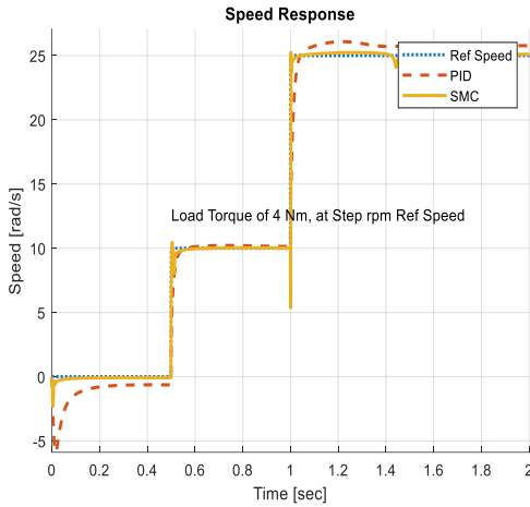
Figure 12. Variable Speed response of PID and SM controller
