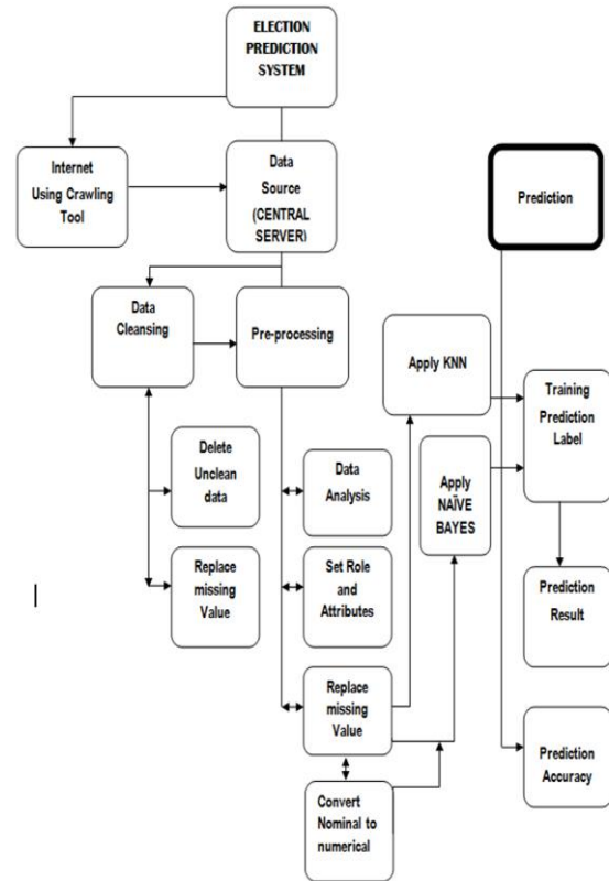
Figure 1: ELECTION TREND PREDICTION SYSTEM
