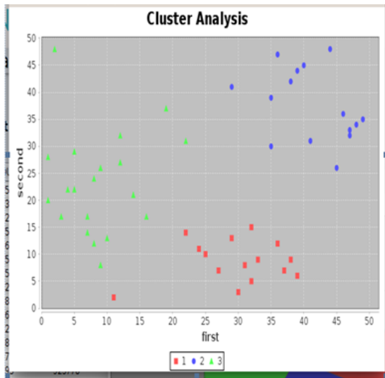
Figure 4: Cluster Analysis
