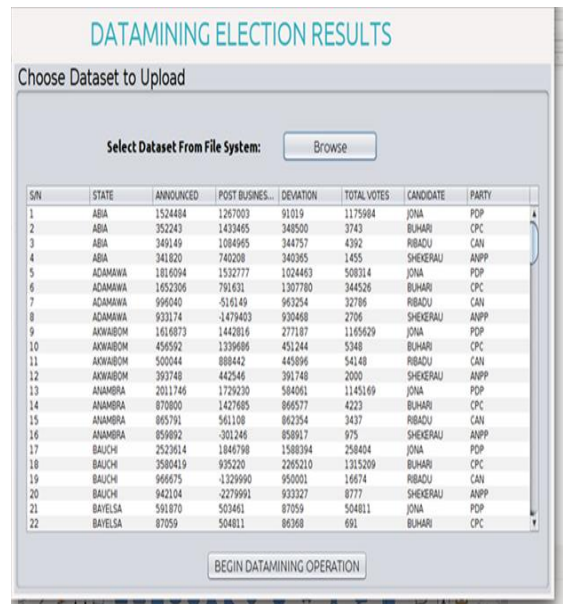
Figure 3: Dataset uploaded
