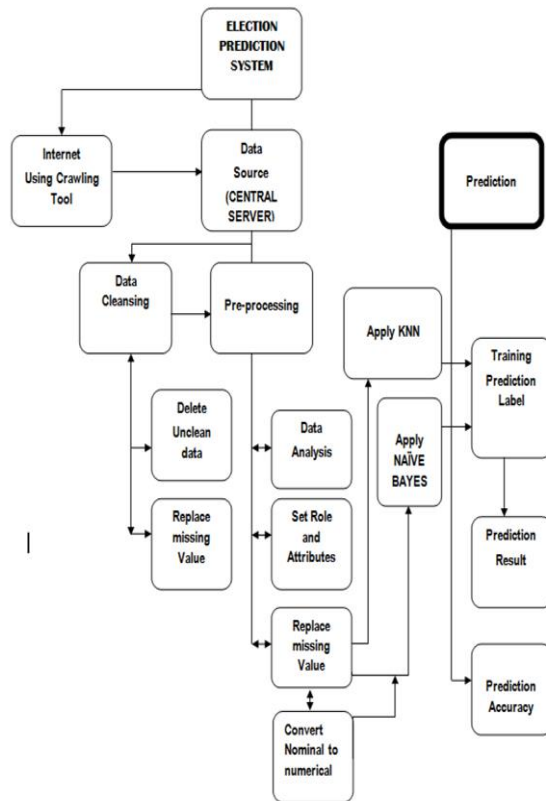
Figure 1: ELECTION TREND PREDICTION SYSTEM
