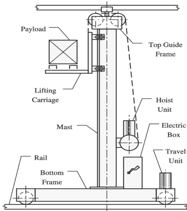
Figure 5: Single-mast stacker crane [18]
