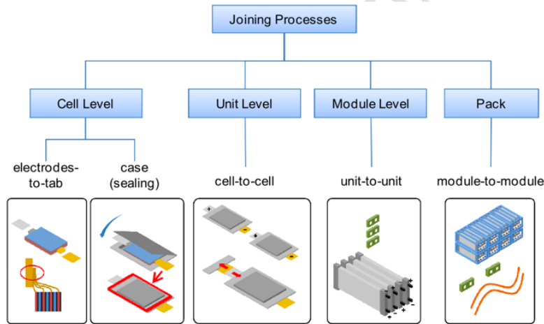
Figure 2: Automotive battery assembly packs
