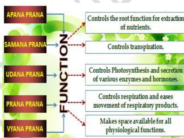
Fig 15 : The Mechanism of Self- Protection in Plant System
