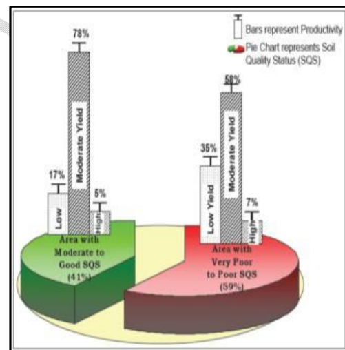
Fig 11 : Yield Performance under varying soil quality in project garden
