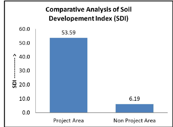
Fig 26 : Soil development index (SDI) indicated the impact of sustainable tea initiative on soil health
