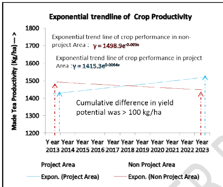
Fig 20 : Exponential trend of change in crop productivity under sustainable tea initiatives in the project garden at Cachar, Assam.
