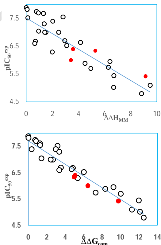
Figure 2. (Top) the equality curve of pIC_{50} and the enthalpy of the coumarin series in the gaseous medium ( \Delta\Delta H_{MM} ) of MAO-B-COUx complex formation; (Below) similar plot for relative \Delta\Delta G_{com} .
