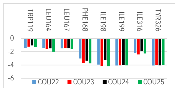
Figure 3. Mechanics intermolecular interaction energy E_{\text{int}} breakdown to residue contributions in the hydrophobic pocket [ \text{kcal.mol}^{-1} ]: (Top) two most active inhibitors COU1-2, (Middle) moderately active inhibitors COU14-15, (Bottom) less active inhibitors COU23-24. Table 2 [11].
