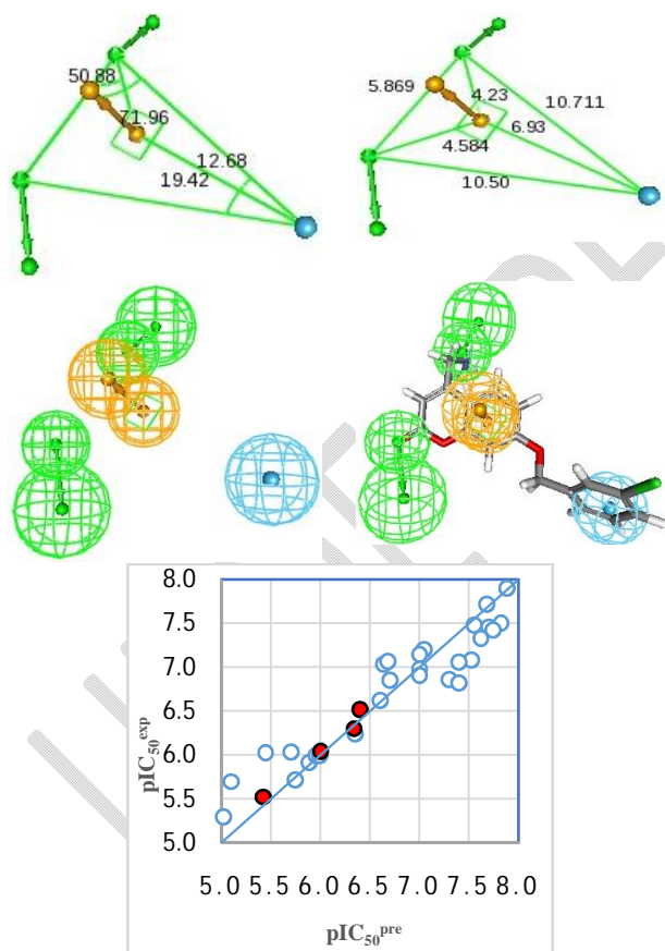
Figure 4. (A, Top left) Angles between centers of pharmacophoric, (B, Top right) distances between centers, (C, Middle left) features coordinates of centers and (D, Middle right) mapping of pharmacophore of MAO-B inhibitor with the most potent molecule COU1. The correlation plot of experimental vs. predicted inhibitory activity is displayed at the left. The features are colored blue for hydrophobic aromatic, green for hydrogen-bond acceptor (HBA) and orange for ring aromatic. The arrows
