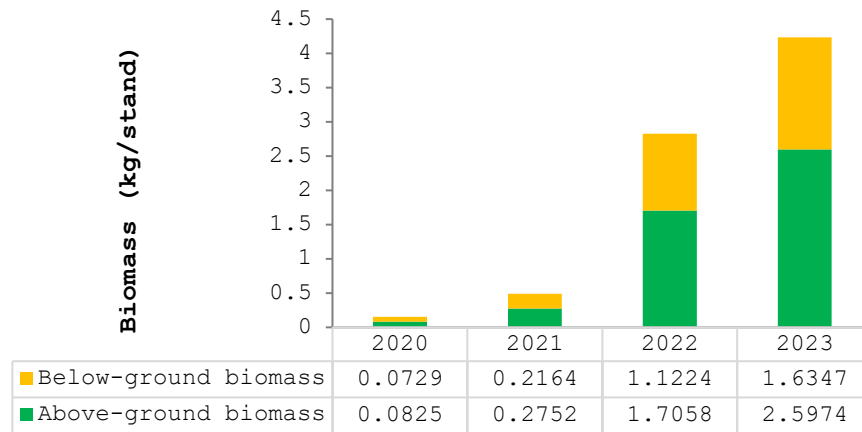
Figure 4. The potential of standing biomass of R. mucronata from the REMAJA PHE ONWJ program in the Pantai Bahagia Village, Bekasi – Indonesia coast.
