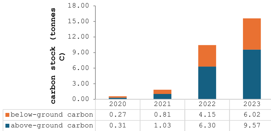
Figure 5. Potential carbon stock of R. mucronata from the REMAJA PHE ONWJ program on the coast of Pantai Bahagia Village, Bekasi – Indonesia.
