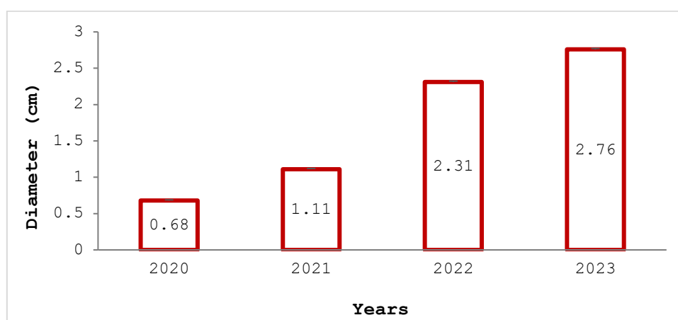
Figure 3. Growth of R. mucronata seedling diameter ( P > 0.05 ) from the REMAJA PHE ONWJ program on the coast of Pantai Bahagia Village, Bekasi – Indonesia
