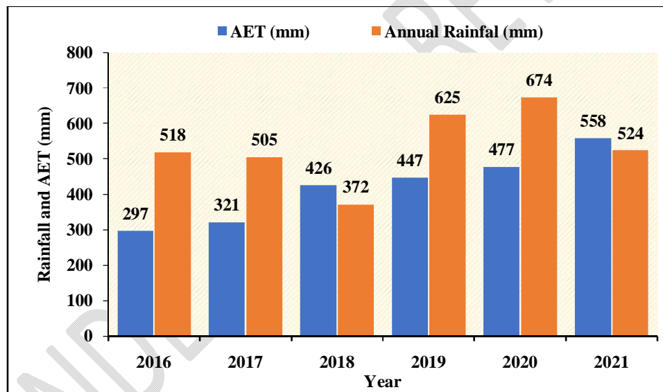
Fig.5. Actual evapotranspiration (AET) and rainfall over different years
