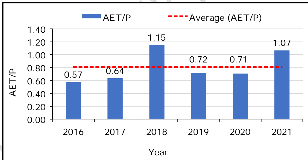
Fig .8. AET/P Ratio of Artal subwatershed of karnatka
