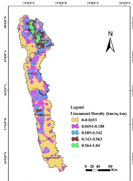
Fig. 5. Spatial distribution map of lineament density
