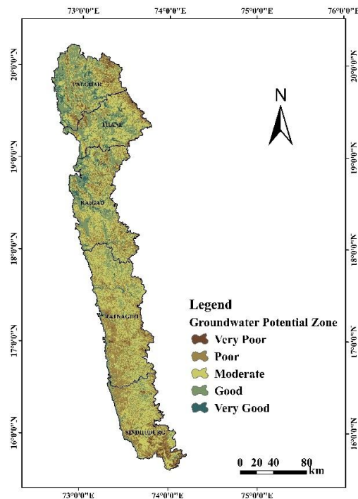
Fig. 11. Spatial distribution map of groundwater potential
