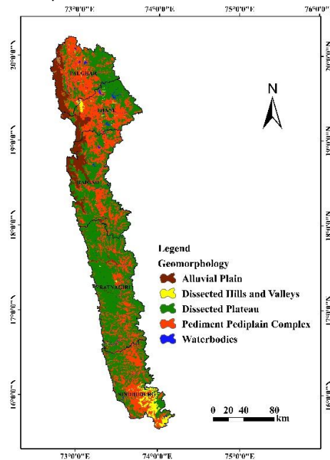
Fig. 4. Spatial distribution map of geomorphology
