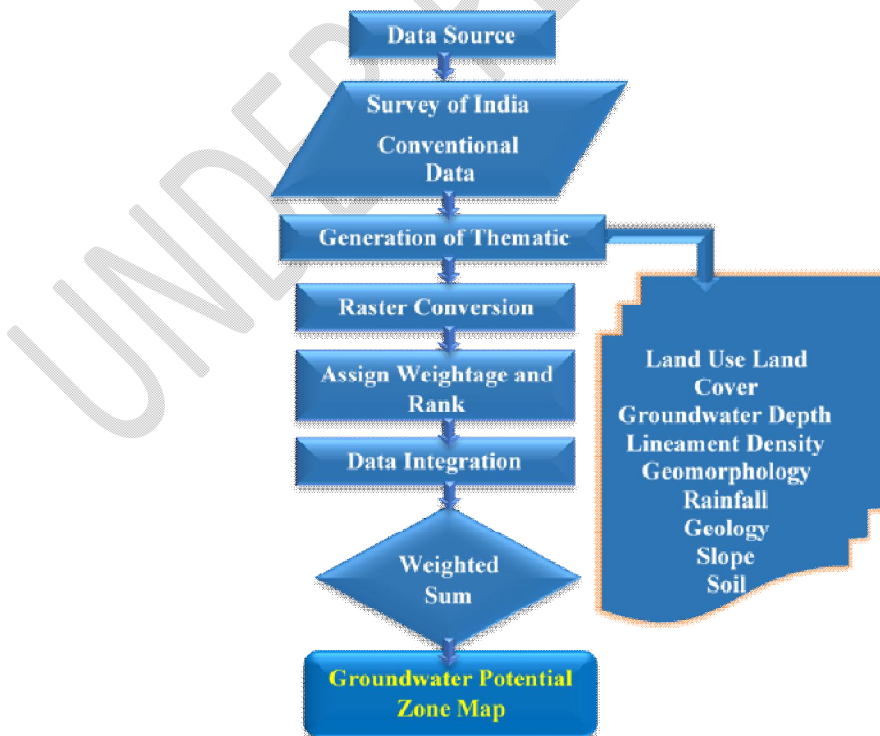
Fig. 2. Flow chart showing steps for preparation of groundwater potential map
