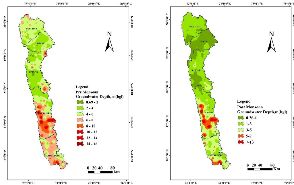
Fig. 10. Spatial distribution of groundwater depth during pre- and post-monsoon periods in the Konkan region
