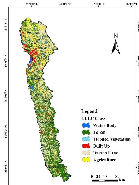
Fig. 9. Spread of LULC classes across all districts of the Konkan region
