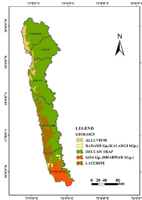
Fig. 3. Spatial distribution map of geology
