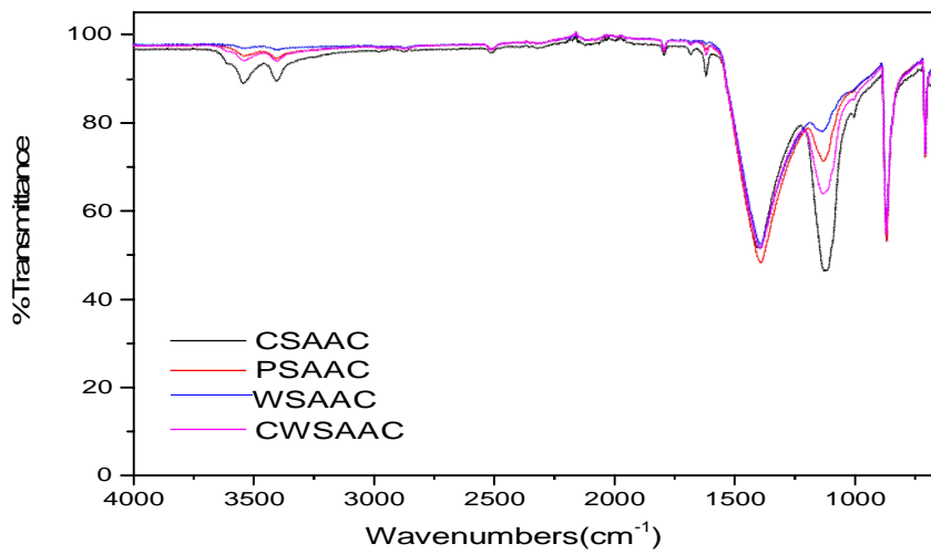
Figure3: Stacked FT-IR spectra of acid-treated activated carbon
