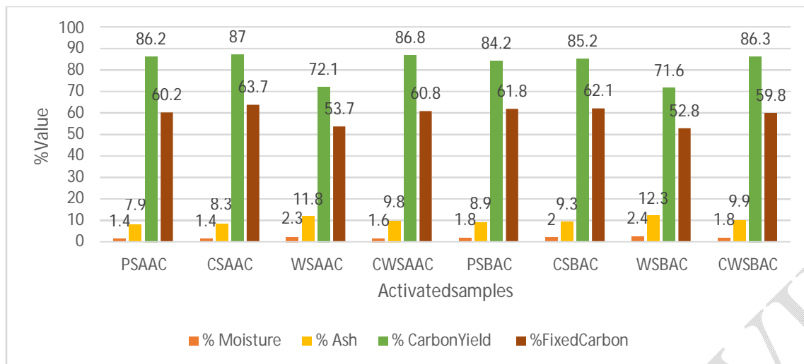
Figure1. Comparison between physicochemical properties of acid-activated carbon and base-activated carbon.
