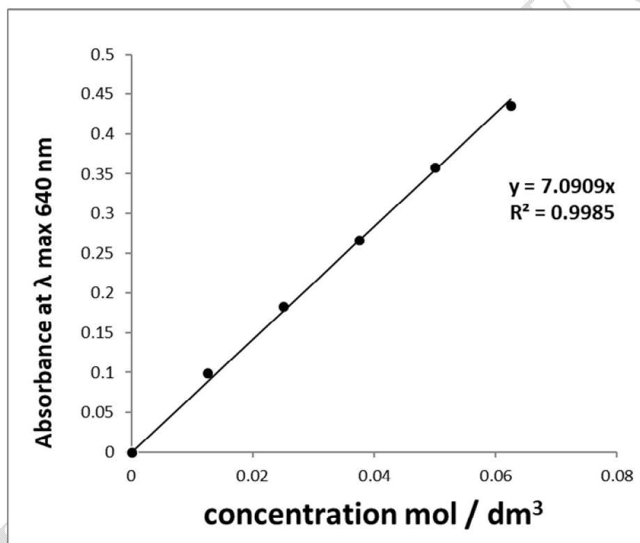
Figure 5 shows the plot of [\text{Ni}(\text{en})]^{2+} complex absorbance versus its concentrations.
