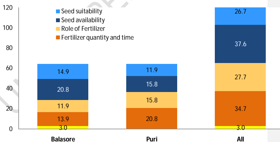
Figure 2. Percentage of topics selected by farmers to receive advisories.
