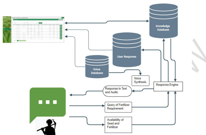
Figure1. Technical Architecture of Chatbot
