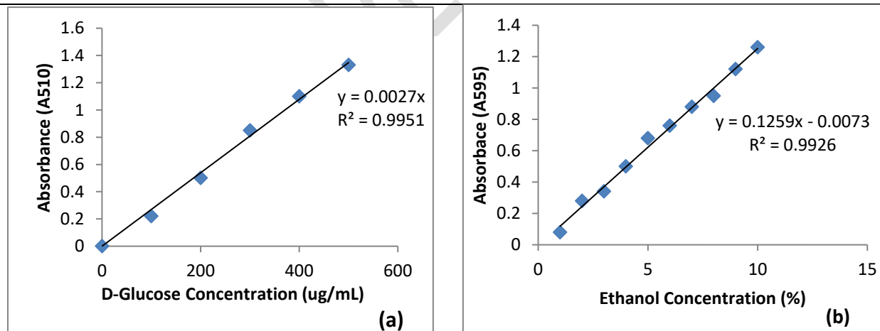
Fig 1. (a) Standard curve for determination of total reducing sugars using 3,5-Dinitrosalicylic acid (DNSA) assay. (b) Standard curve for determination of ethanol concentration using dichromatic oxidation reaction.
