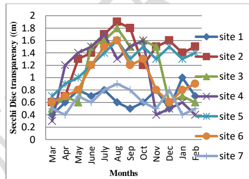
Fig. 5, showing monthly variation in Secchi Disc transparency (m) at different sites of Dal lake.
