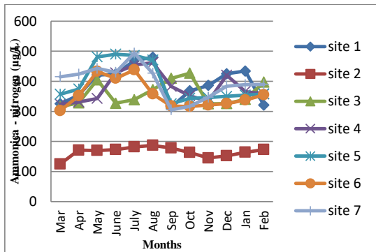
Fig. 14, showing monthly variation in Ammoniacal-nitrogen ( \mu\text{g/L} ) at different sites of Dal lake.
