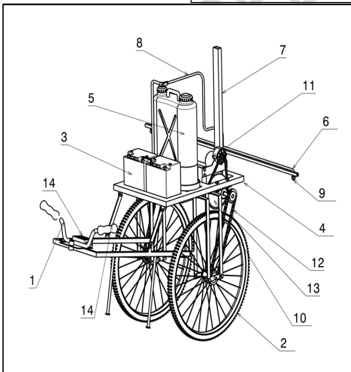
Fig.1 Schematic diagram of developed battery-operated boom sprayer
