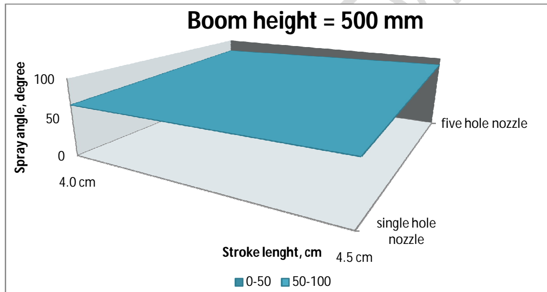
Fig.12 Effect of different types of nozzles at different stroke length on angle of spray at 500 mm boom height
