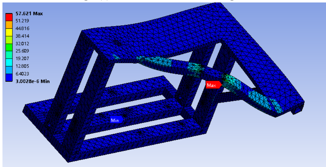
Fig. 9(b) Equivalent stress cloud diagram
