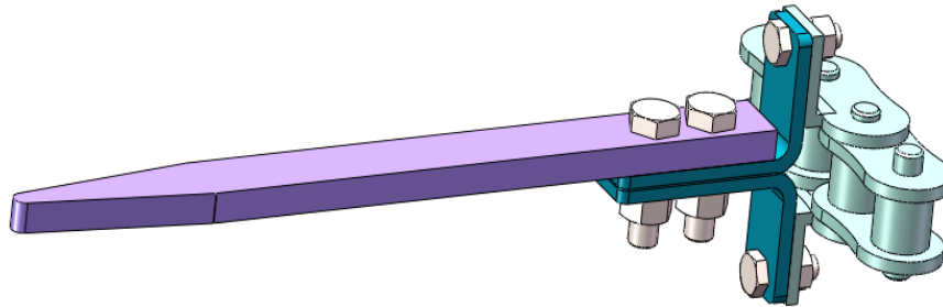
Fig. 4. Actuating device
