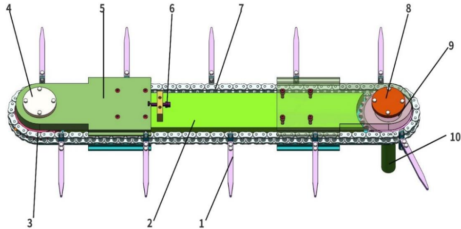
1. Rake tooth 2. Connecting frame 3. Idler sprocket 4. Bearing cover 5. Top cover 6. Adjusting bolt 7. Chain 8. Self-aligning roller bearing 9. Drive sprocket 10. Drive shaft. Fig. 3. Conveying System
