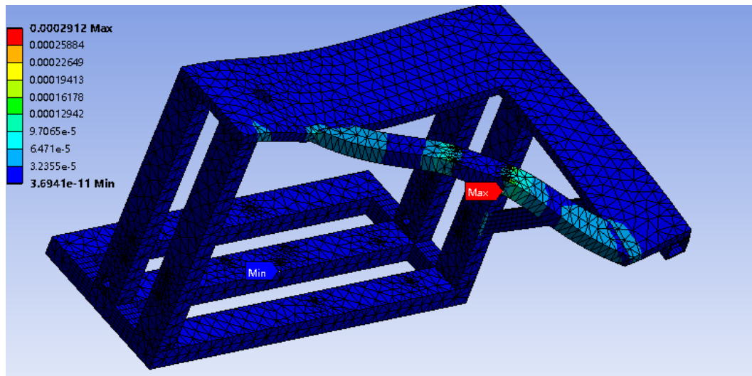
Fig. 9(a) Total deformation cloud diagram
