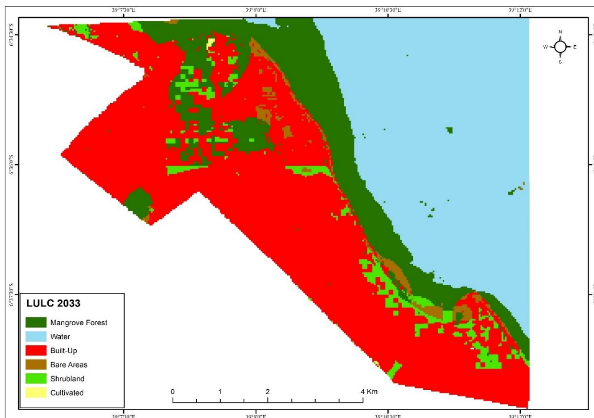
Figure 3: LULC for the year 2033
