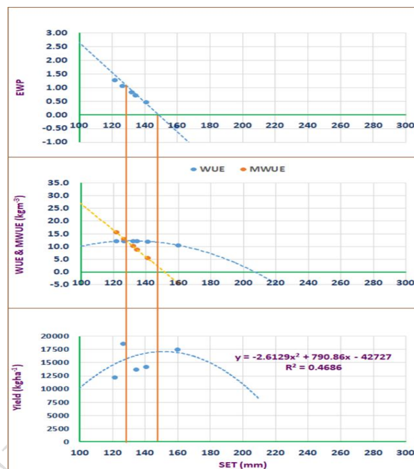
Fig. 5. Relation of yield, WUE and MWUE against ET for a quadratic ET production function for net head yield of broccoli grown under black polyethylene mulch condition (averaged over irrigation regimes).
