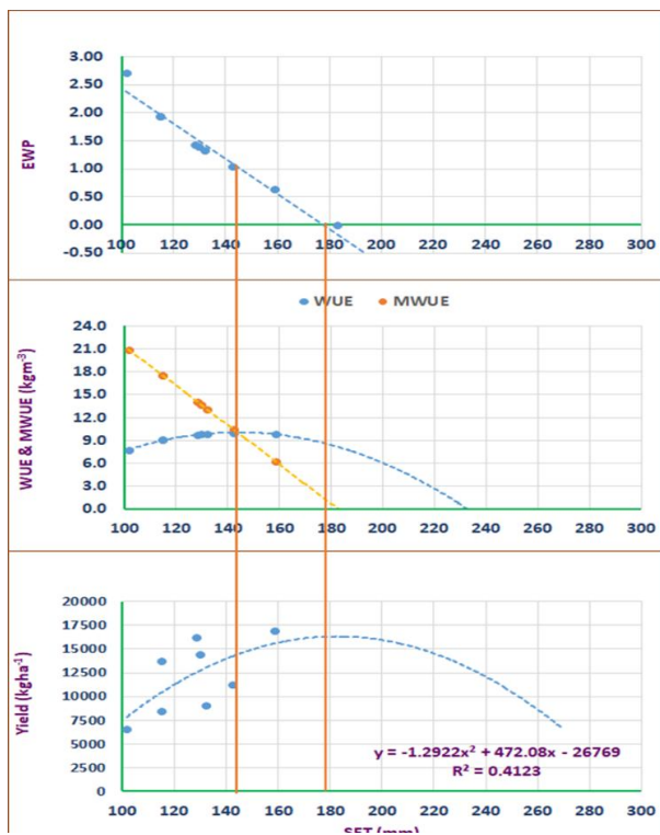
Fig. 6. Relation of yield, WUE and MWUE against ET for a quadratic ET production function for net head yield of broccoli grown under paddy straw mulchcondition (averaged over irrigation regimes).
