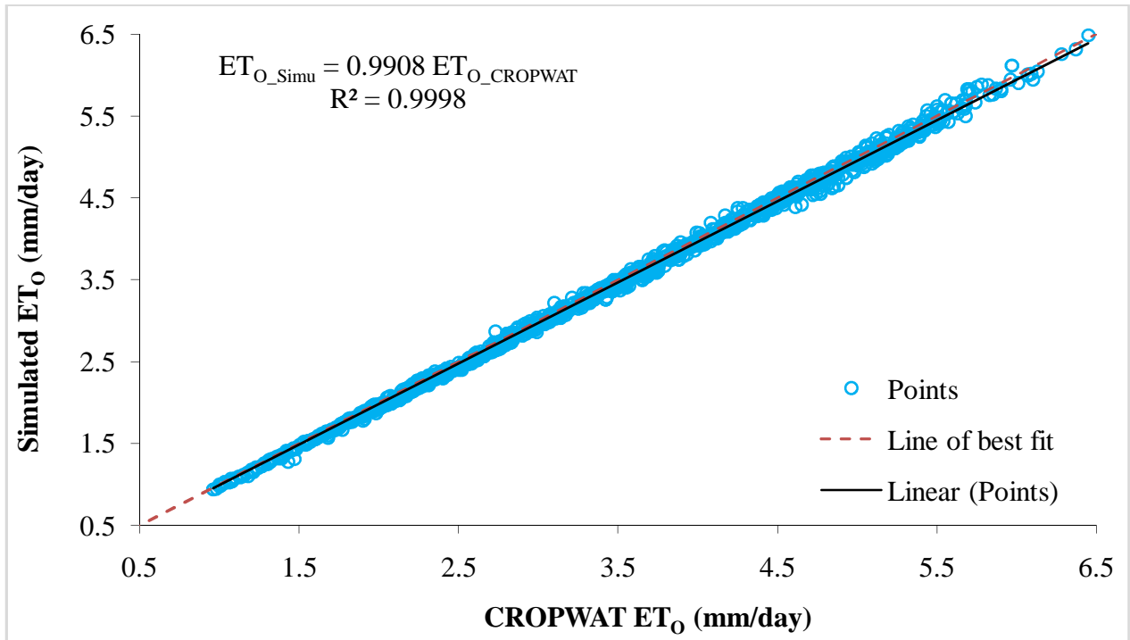
Fig. 2: Scatter plot of simulated and CROPWAT estimated daily ET_0 estimates during the years from 2020 to 2022 over SHUATS, Prayagraj.
