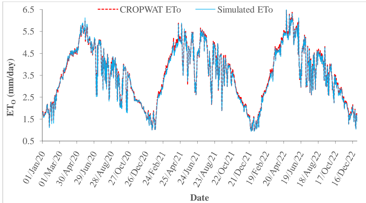
Fig. 2: Daily time series of simulated and CROPWAT determined ET_0 estimates during the years from 2020 to 2022 over SHUATS, Prayagraj.
