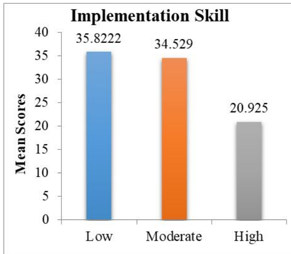
Fig. 2. Implementation Skill
