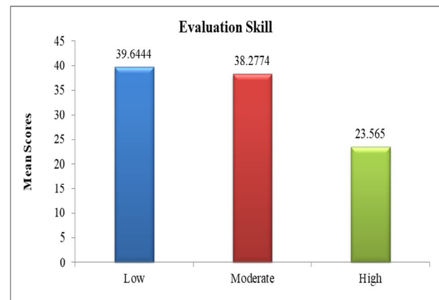
Fig. 4. Evaluation Skill
