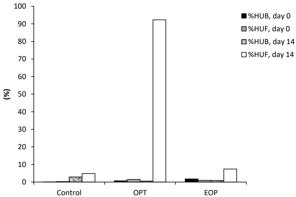
Figure 3: Proportion (%) of THB and TF that are HUB and HUF respectively.
