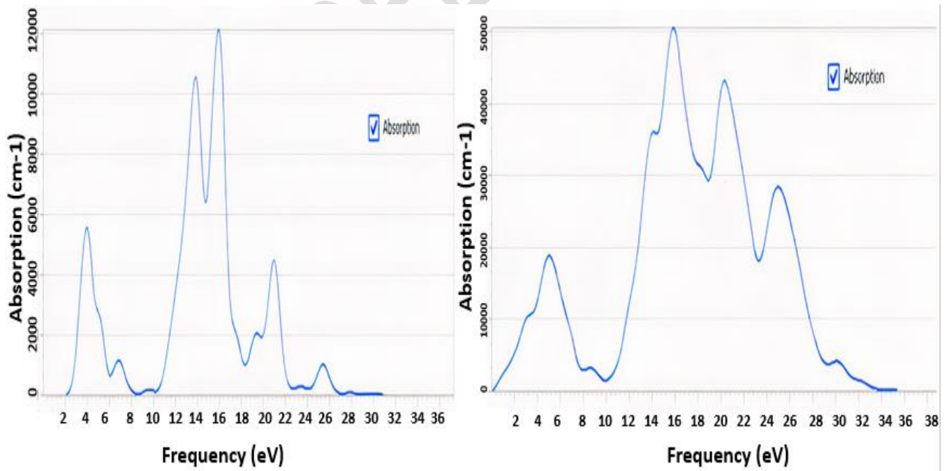
Figure 4: (a) Absorption of Monolayer and (b) Bilayer with vacancy
