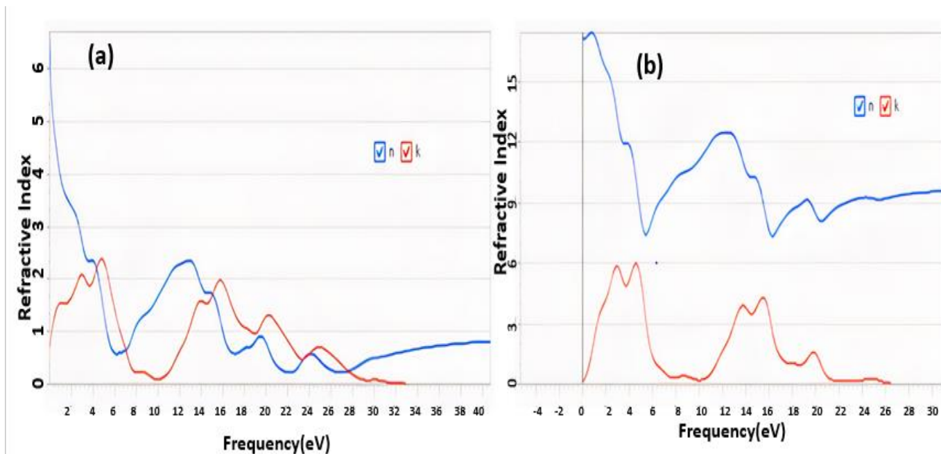
Figures 3: (a) Refractive index of Monolayer with vacancy, (b) Monolayer doped with Phosphorous
