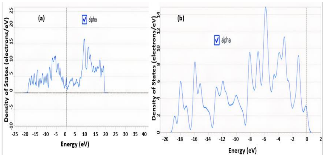
Figures 2: (a) Density of State of Bilayer with Vacancy and, (b) Monolayer doped with Aluminium
