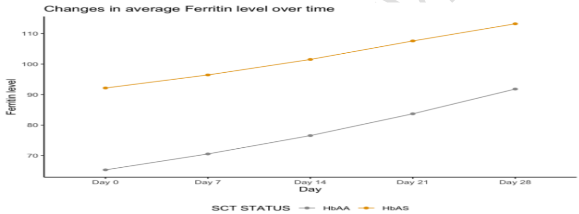
Figure 8: Changes in average Ferritin level (ng/ml) over time (day 0-day 28) for both Sickle cell trait donor(HbAS) blood and sickle cell trait negative (Hb AA) donor blood.
