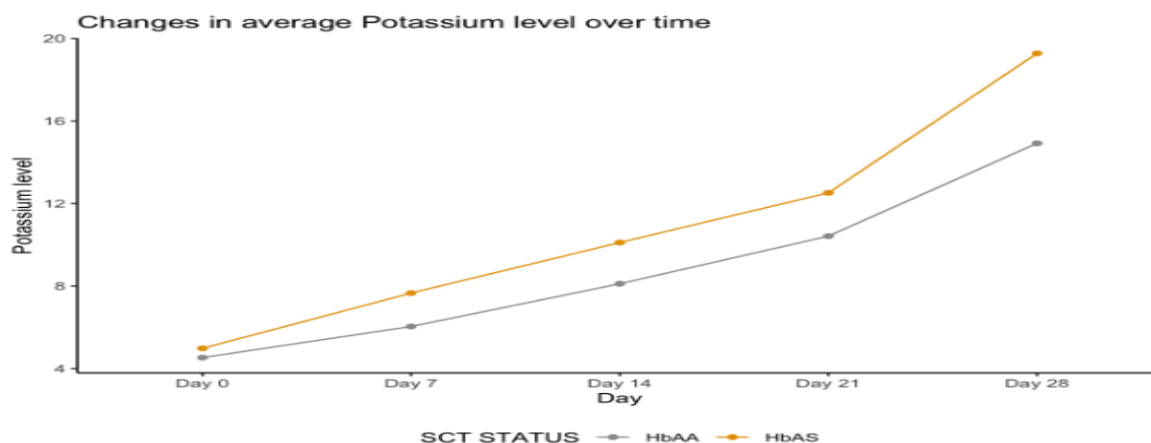
Figure 10: changes in average Potassium level (mmol/L) over time (day 0-day 28) for both Sickle cell trait donor(HbAS) blood and sickle cell trait negative (Hb AA) donor blood.
