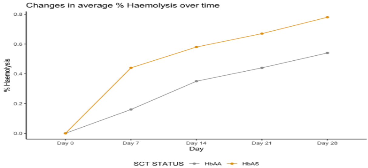
Figure 1: changes in average percentage Haemolysis (%) over time (day 0-day 28) for both Sickle cell trait donor(HbAS) blood and sickle cell trait negative (Hb AA) donor blood.
