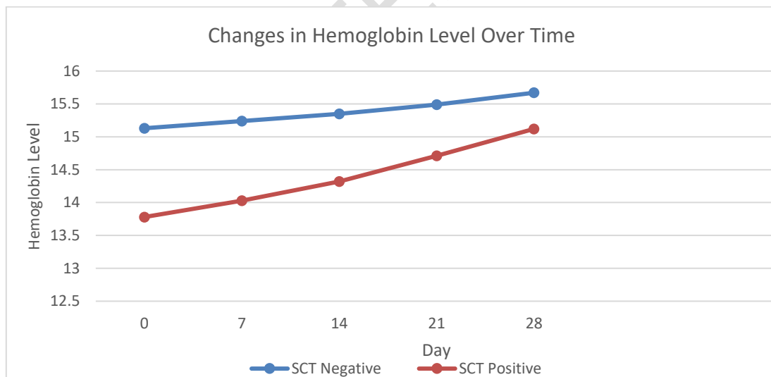
Figure 6: changes in average Haemoglobin level over time for both Sickle cell trait donor(HbAS) blood and sickle cell trait negative (Hb AA) donor blood.
