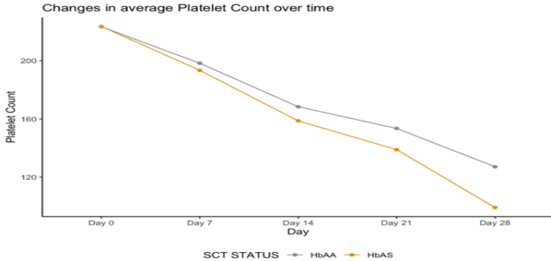
Figure 5: changes in average platelet count over time for both Sickle cell trait donor(HbAS) blood and sickle cell trait negative (Hb AA) donor blood.
