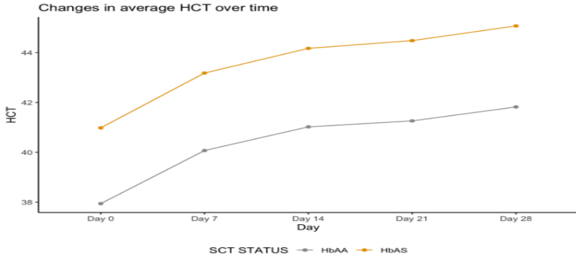
Figure 3: changes in average Hematocrit (%) over time (day 0-day 28) for both Sickle cell trait donor(HbAS) blood and sickle cell trait negative (Hb AA) donor blood
