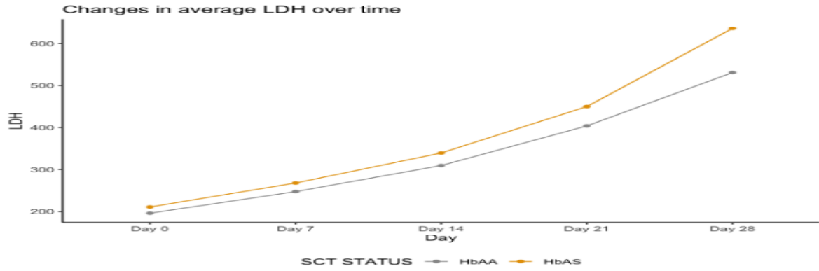
Figure 7: Changes in average Lactate dehydrogenase(U/L) over time (day 0-day 28) for both Sickle cell trait donor(HbAS) blood and sickle cell trait negative (Hb AA) donor blood.
