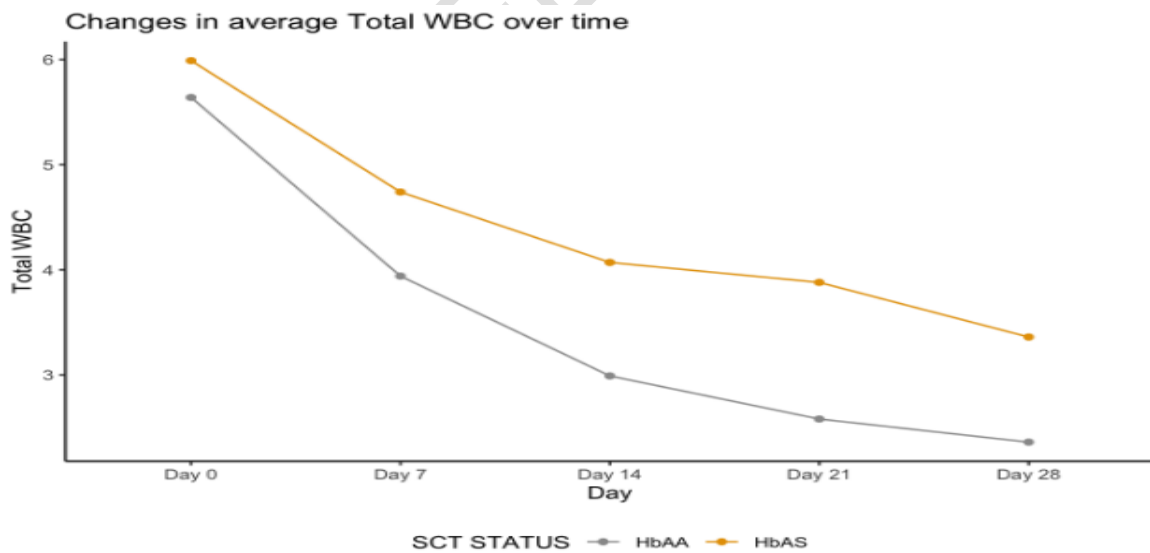
Figure 4: changes in average Total white blood cells ( \times 10^9/L ) over time (day 0-day 28) for both Sickle cell trait donor(HbAS) blood and sickle cell trait negative (Hb AA) donor blood.
