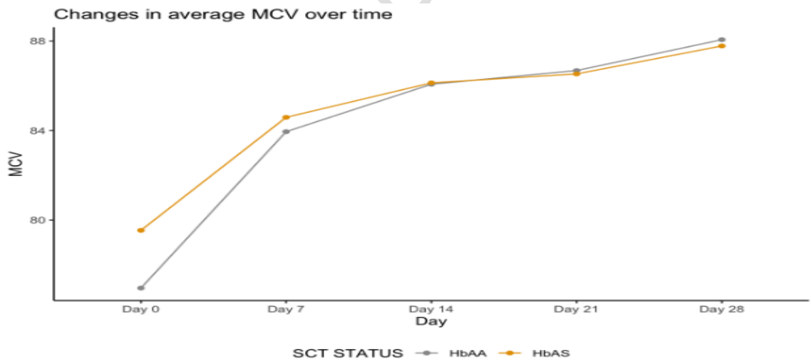
Figure 2: changes in average Mean cell volume(fL) over time (day 0-day 28) for both Sickle cell trait donor(HbAS) blood and sickle cell trait negative (Hb AA) donor blood
