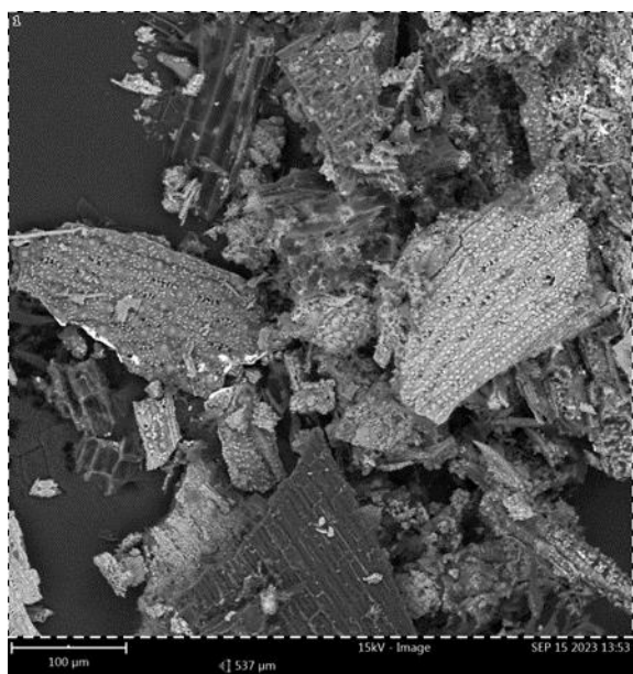
Fig.4a SEM of rice straw biochar
