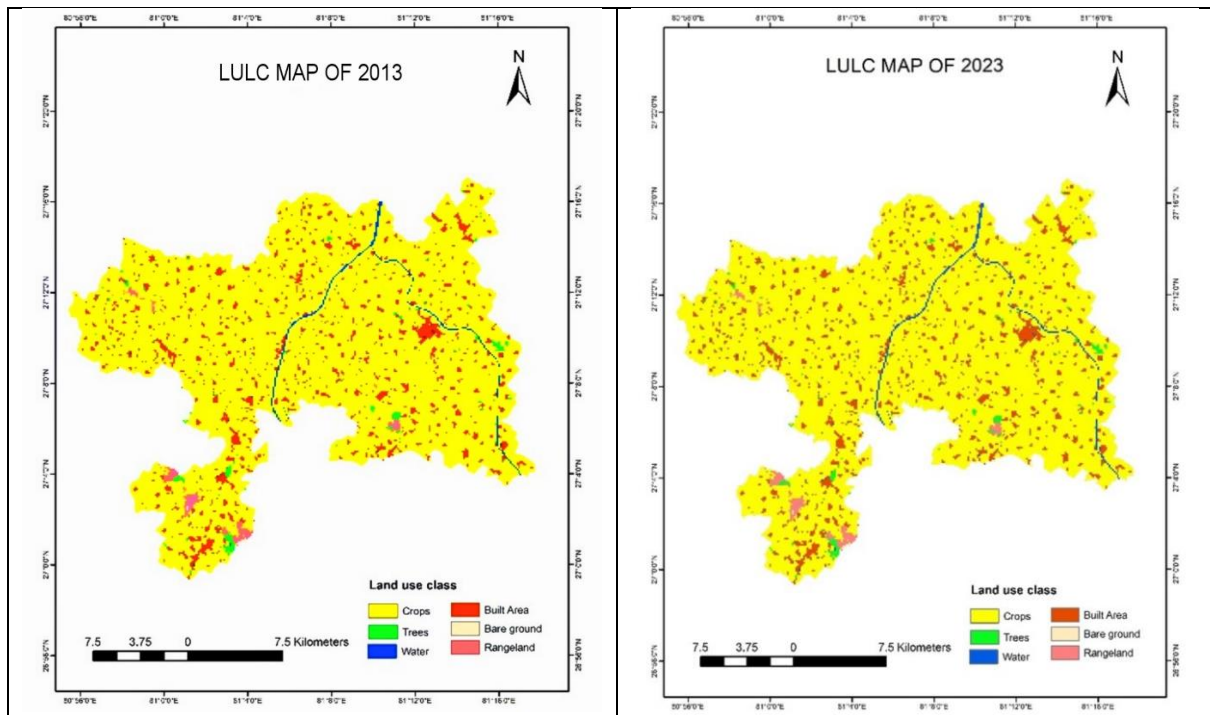
Fig. 3 LULC maps of 2013 and 2023
