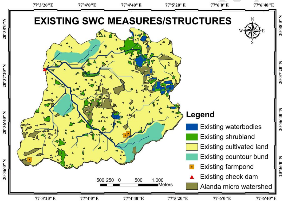
Fig. 2 Existing SWC measures/structures in Alanda micro watershed
